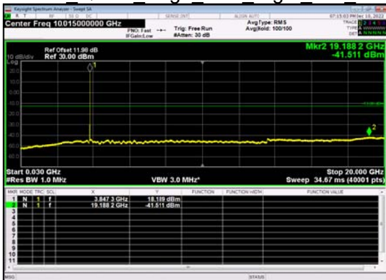
N77(15M)_DFT-s- OFDM QPSK Edge 1RB Right Mid CH
