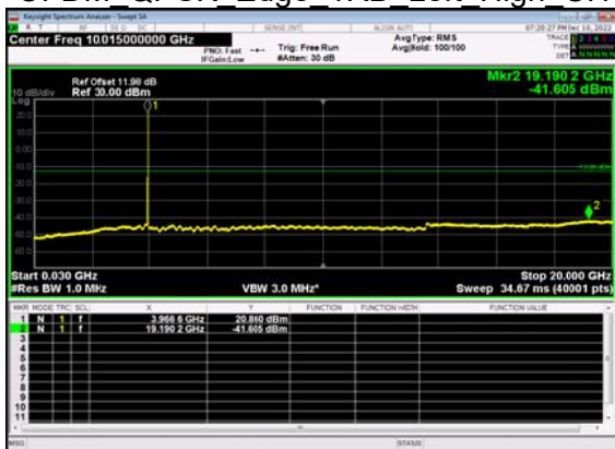
N77(15M)_DFT-s- OFDM QPSK Edge 1RB Left High CH
