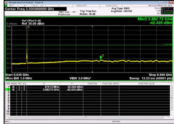
N71(20M)_DFT-s- OFDM BPSK Edge 1RB Left High CH
