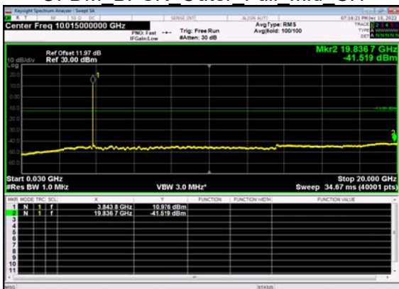
N77(15M)_DFT-s- OFDM BPSK Outer Full Mid CH
