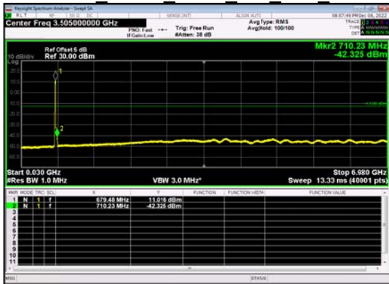
N71(20M)_DFT-s- OFDM QPSK Outer Full Low CH
