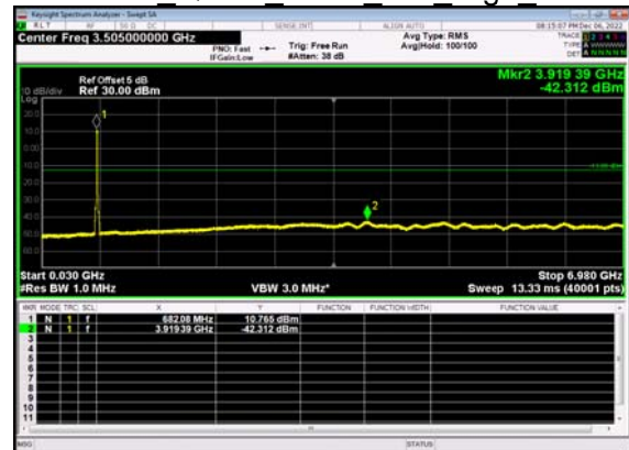
N71(20M)_DFT-s- OFDM QPSK Outer Full High CH
