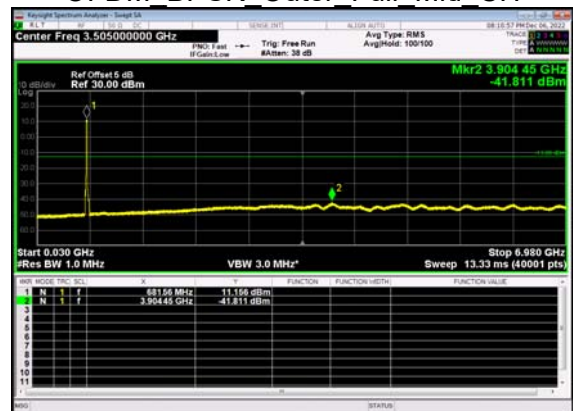
N71(20M)_DFT-s- OFDM BPSK Outer Full Mid CH
