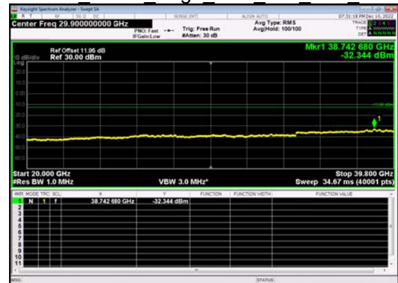
N77(20M)_DFT-s- OFDM BPSK Edge 1RB Left Low CH
