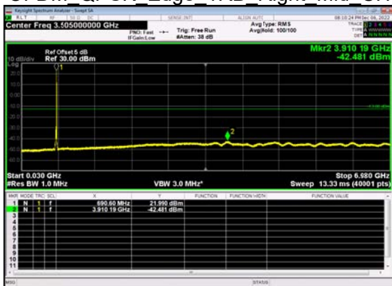
N71(20M)_DFT-s- OFDM QPSK Edge 1RB Right Mid CH
