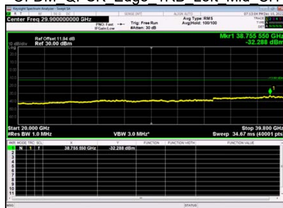
N77(15M)_DFT-s- OFDM QPSK Edge 1RB Left Mid CH
