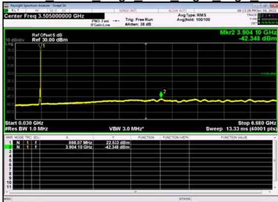
N71(20M)_DFT-s- OFDM BPSK Edge 1RB Right High CH
