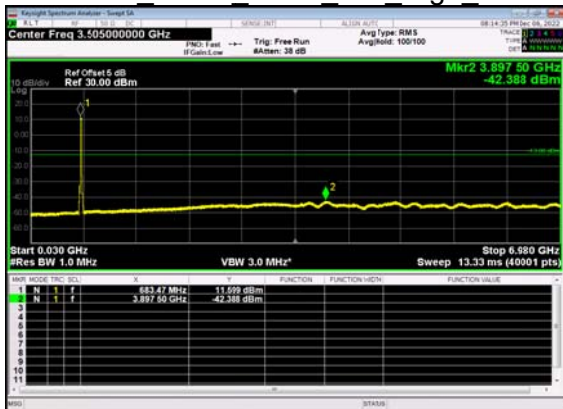
N71(20M)_DFT-s- OFDM BPSK Outer Full High CH
