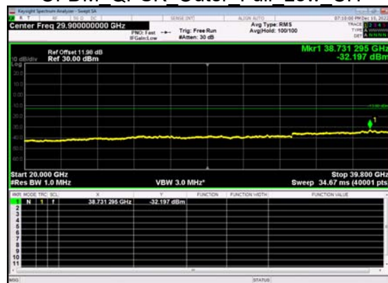
N77(15M)_DFT-s- OFDM QPSK Outer Full Low CH
