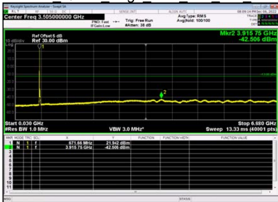
N71(20M)_DFT-s- OFDM QPSK Edge 1RB Left Mid CH
