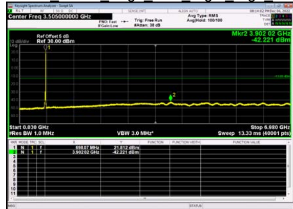
N71(20M)_DFT-s- OFDM QPSK Edge 1RB Right High CH
