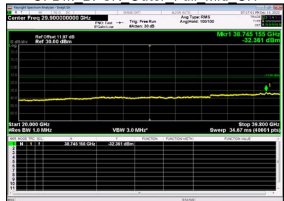
N77(15M)_DFT-s- OFDM BPSK Outer Full Mid CH
