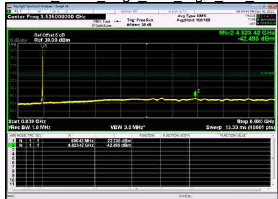
N71(20M)_DFT-s- OFDM BPSK Edge 1RB Right Mid CH
