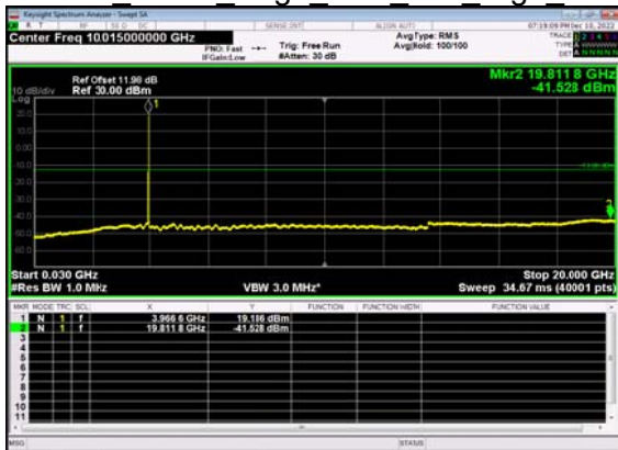
N77(15M)_DFT-s- OFDM BPSK Edge 1RB Left High CH
