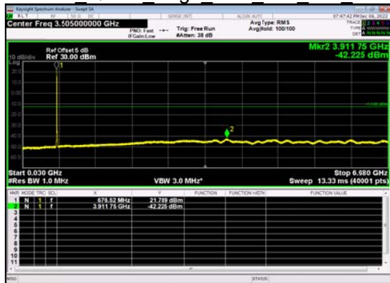
N71(10M)_DFT-s- OFDM QPSK Edge 1RB Left Mid CH
