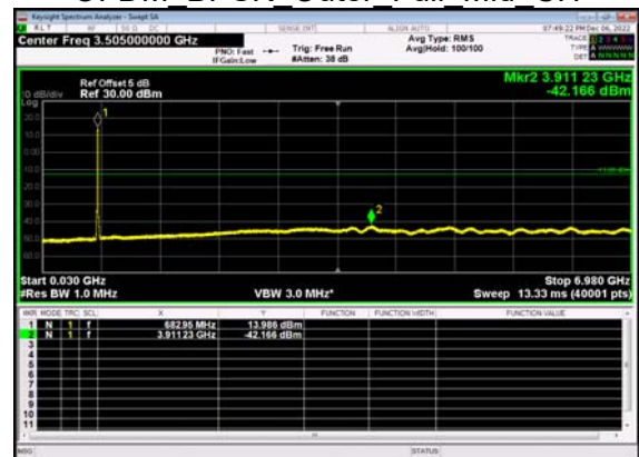
N71(10M)_DFT-s- OFDM BPSK Outer Full Mid CH
