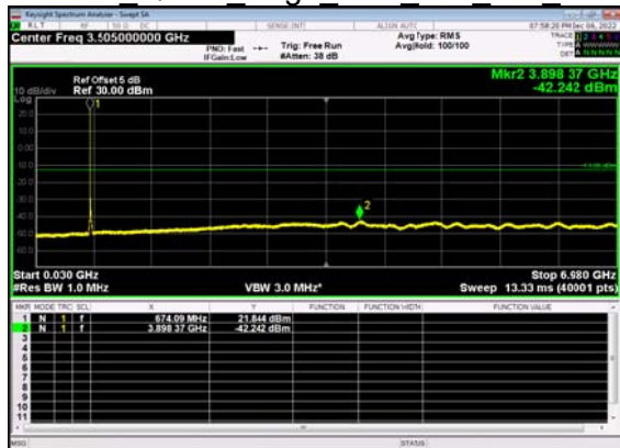
N71(15M)_DFT-s- OFDM QPSK Edge 1RB Left Mid CH
