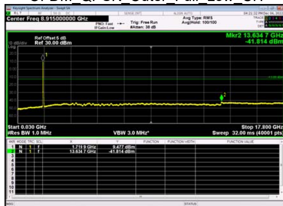
N66(25M)_DFT-s- OFDM QPSK Outer Full Low CH
