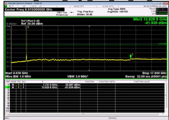
N66(30M)_DFT-s- OFDM QPSK Edge 1RB Left Mid CH
