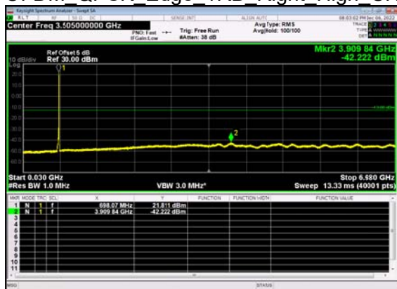
N71(15M)_DFT-s- OFDM QPSK Edge 1RB Right High CH
