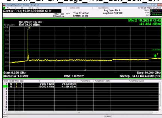
N41(90M)_DFT-s- OFDM QPSK Edge 1RB Left Low CH
