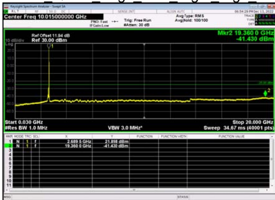
N41(80M)_DFT-s- OFDM QPSK Edge 1RB Right High CH
