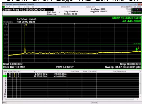
N41(90M)_DFT-s- OFDM QPSK Edge 1RB Left Mid CH
