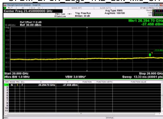
N41(90M)_DFT-s- OFDM BPSK Edge 1RB Left Mid CH
