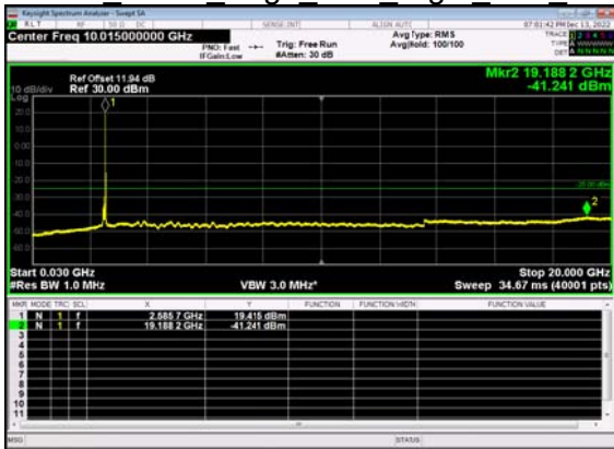
N41(90M)_DFT-s- OFDM BPSK Edge 1RB Right Low CH
