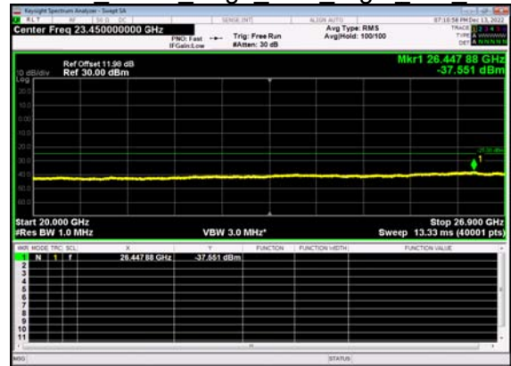
N41(90M)_DFT-s- OFDM BPSK Edge 1RB Right Mid CH
