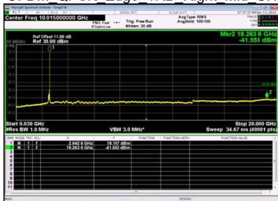
N41(100M)_DFT-s- OFDM QPSK Edge 1RB Right Mid CH
