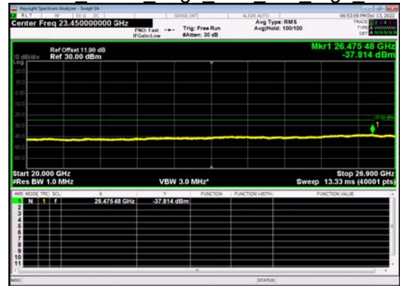
N41(80M)_DFT-s- OFDM QPSK Edge 1RB Left High CH
