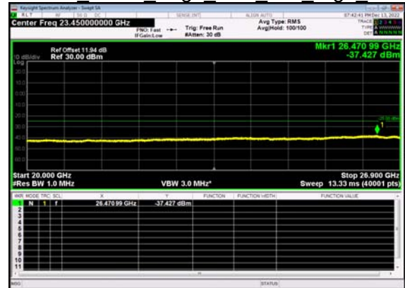
N41(100M)_DFT-s- OFDM BPSK Edge 1RB Left High CH
