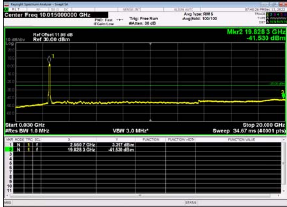
N41(100M)_DFT-s- OFDM QPSK Outer Full Mid CH
