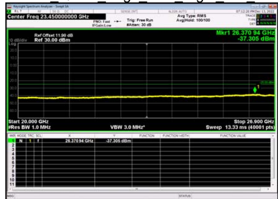
N41(90M)_DFT-s- OFDM QPSK Edge 1RB Right Mid CH
