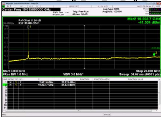
N41(80M)_DFT-s- OFDM QPSK Edge 1RB Left High CH
