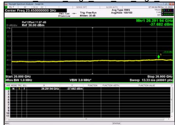
N41(100M)_DFT-s- OFDM QPSK Edge 1RB Left High CH
