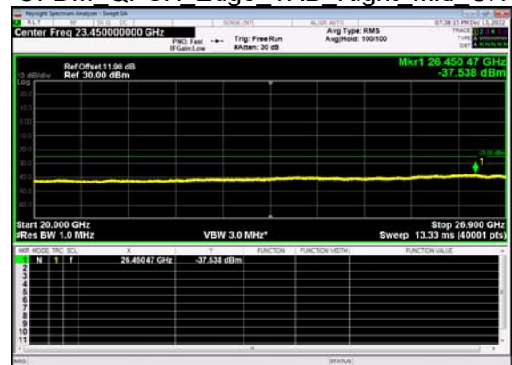
N41(100M)_DFT-s- OFDM QPSK Edge 1RB Right Mid CH
