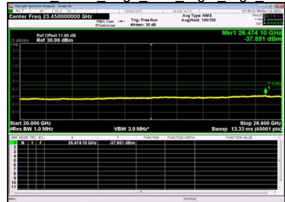
N41(100M)_DFT-s- OFDM BPSK Edge 1RB Right High CH
