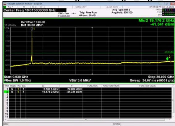
N41(100M)_DFT-s- OFDM BPSK Edge 1RB Right High CH
