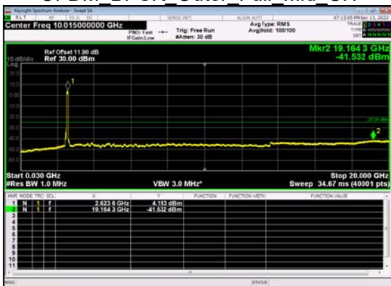
N41(90M)_DFT-s- OFDM BPSK Outer Full Mid CH
