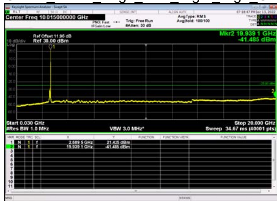
N41(90M)_DFT-s- OFDM BPSK Edge 1RB Right High CH
