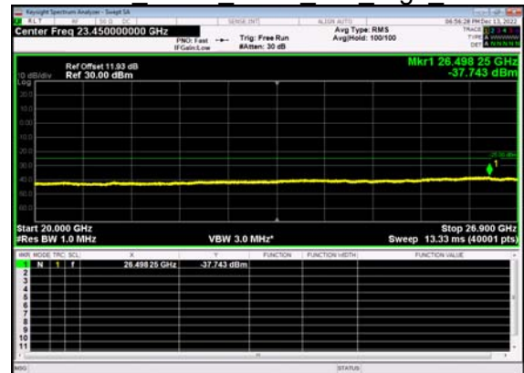
N41(80M)_DFT-s- OFDM BPSK Outer Full High CH
