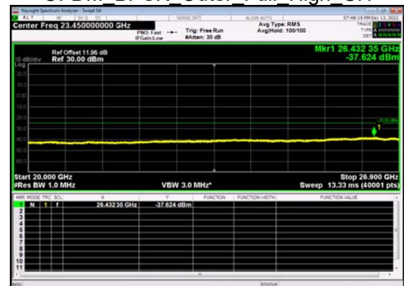
N41(100M)_DFT-s- OFDM BPSK Outer Full High CH
