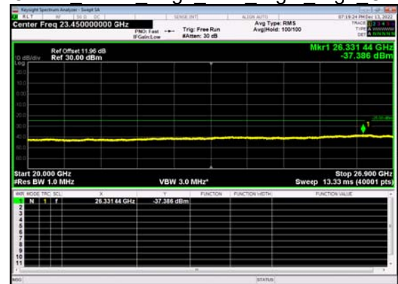
N41(90M)_DFT-s- OFDM BPSK Edge 1RB Right High CH
