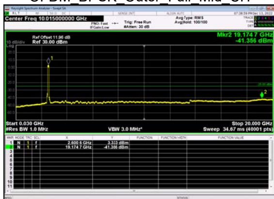
N41(100M)_DFT-s- OFDM BPSK Outer Full Mid CH
