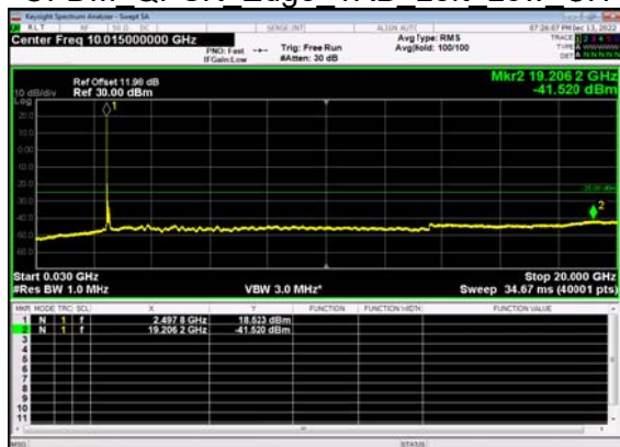
N41(100M)_DFT-s- OFDM QPSK Edge 1RB Left Low CH
