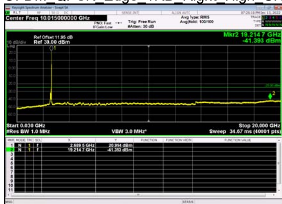
N41(90M)_DFT-s- OFDM QPSK Edge 1RB Right High CH
