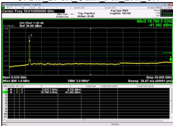
N41(100M)_DFT-s-OFDM BPSK Outer Full Low CH
