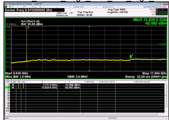
N66(10M)_DFT-s- OFDM QPSK Edge 1RB Left High CH
