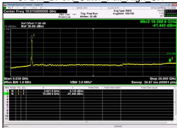
N41(90M)_DFT-s- OFDM BPSK Outer Full High CH
