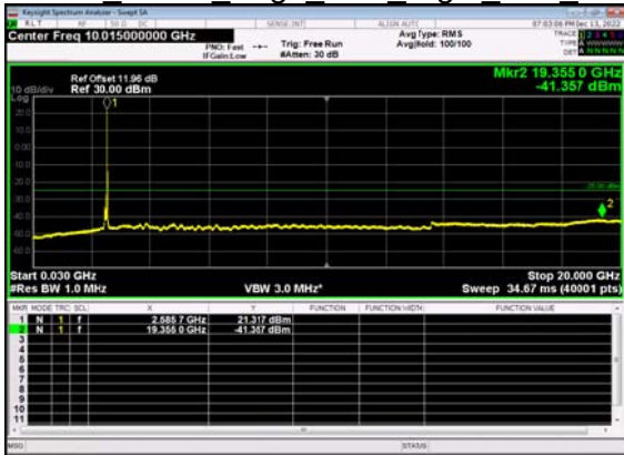
N41(90M)_DFT-s- OFDM QPSK Edge 1RB Right Low CH
