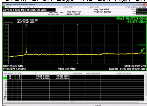
N41(90M)_DFT-s- OFDM QPSK Edge 1RB Left High CH
