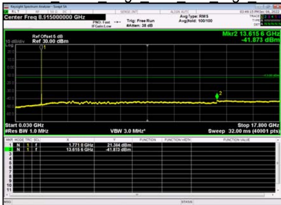
N66(10M)_DFT-s- OFDM BPSK Edge 1RB Left High CH
