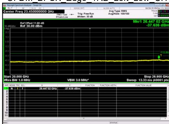
N41(90M)_DFT-s- OFDM BPSK Edge 1RB Left Low CH
