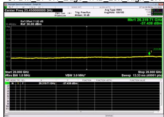
N41(90M)_DFT-s- OFDM BPSK Edge 1RB Left High CH
