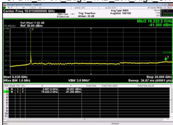
N41(90M)_DFT-s- OFDM BPSK Edge 1RB Left High CH
