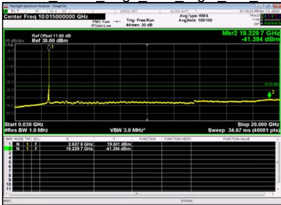
N41(90M)_DFT-s- OFDM BPSK Edge 1RB Right Mid CH
