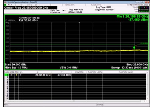
N41(100M)_DFT-s- OFDM QPSK Outer Full Mid CH
