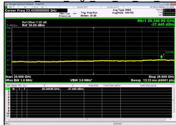
N41(100M)_DFT-s- OFDM BPSK Edge 1RB Left Low CH
