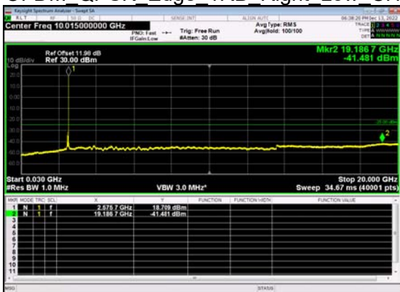
N41(80M)_DFT-s- OFDM QPSK Edge 1RB Right Low CH
