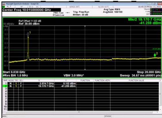
N41(80M)_DFT-s- OFDM QPSK Outer Full Mid CH
