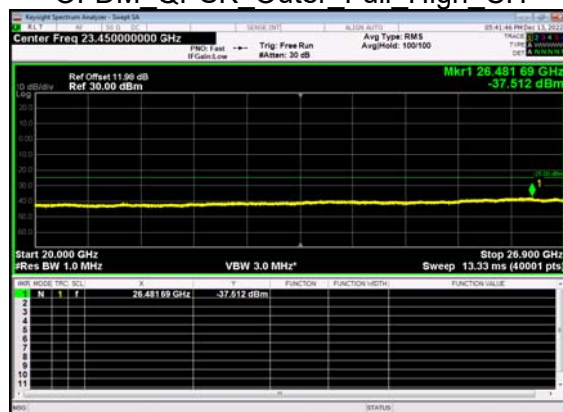
N41(40M)_DFT-s- OFDM QPSK Outer Full High CH
