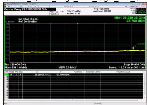
N41(60M)_DFT-s- OFDM QPSK Edge 1RB Right Mid CH
