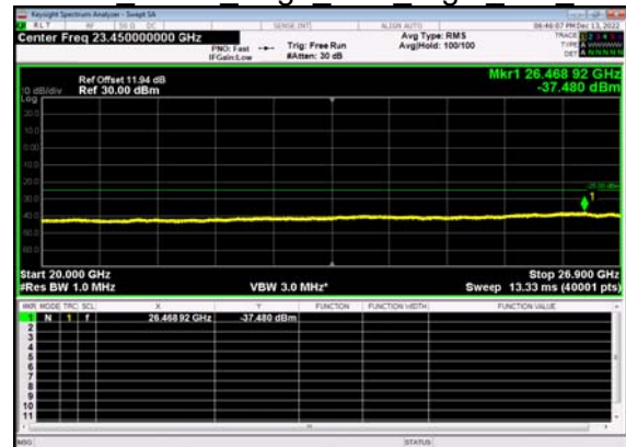
N41(80M)_DFT-s- OFDM BPSK Edge 1RB Right Mid CH
