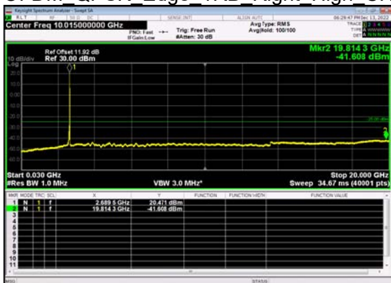
N41(60M)_DFT-s- OFDM QPSK Edge 1RB Right High CH
