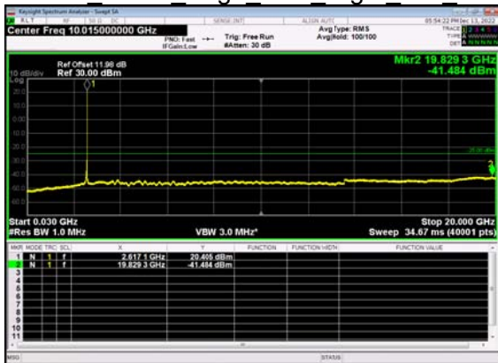
N41(50M)_DFT-s- OFDM BPSK Edge 1RB Right Mid CH
