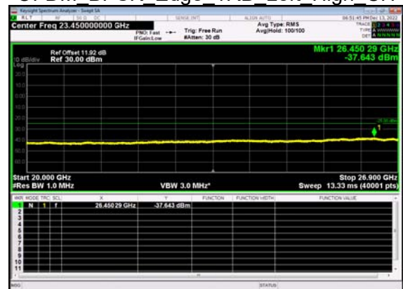
N41(80M)_DFT-s- OFDM BPSK Edge 1RB Left High CH
