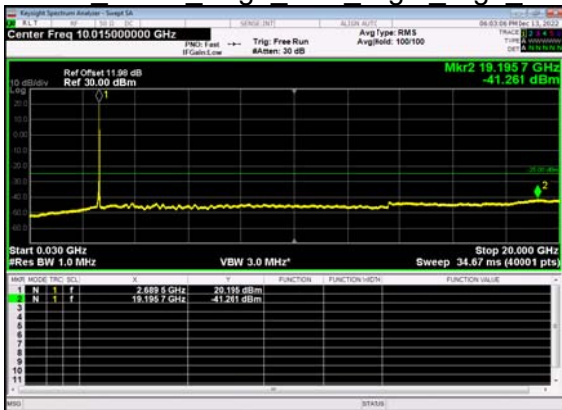
N41(50M)_DFT-s- OFDM BPSK Edge 1RB Right High CH
