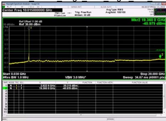
N41(60M)_DFT-s- OFDM BPSK Edge 1RB Right Mid CH
