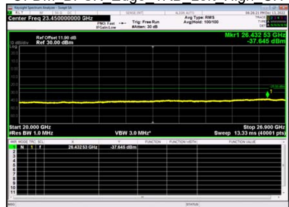
N41(60M)_DFT-s- OFDM BPSK Edge 1RB Left High CH
