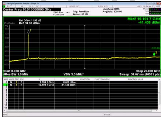
N41(40M)_DFT-s- OFDM BPSK Outer Full Mid CH
