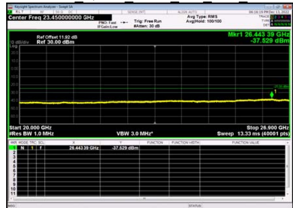
N41(60M)_DFT-s- OFDM QPSK Outer Full Low CH
