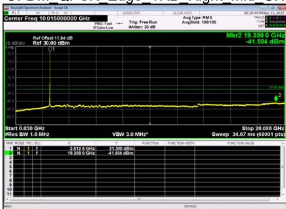
N41(40M)_DFT-s- OFDM QPSK Edge 1RB Right Mid CH
