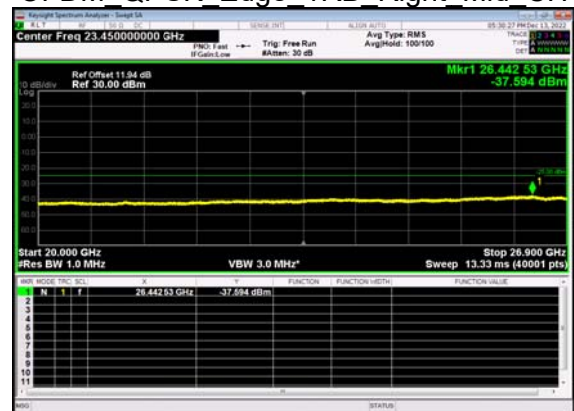
N41(40M)_DFT-s- OFDM QPSK Edge 1RB Right Mid CH
