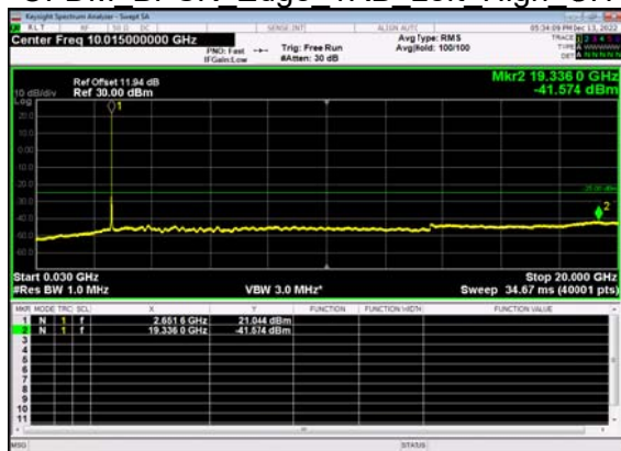
N41(40M)_DFT-s- OFDM BPSK Edge 1RB Left High CH
