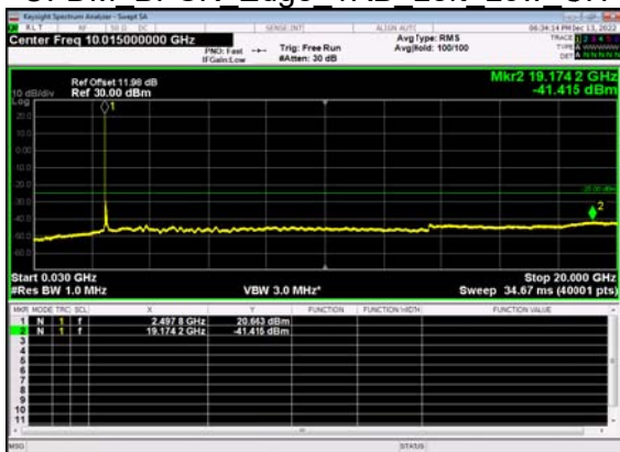
N41(80M)_DFT-s- OFDM BPSK Edge 1RB Left Low CH
