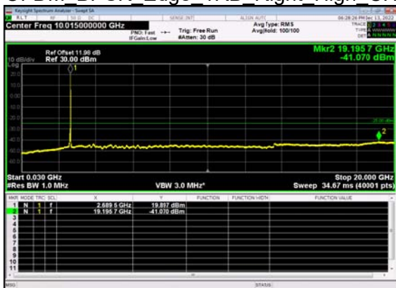
N41(60M)_DFT-s- OFDM BPSK Edge 1RB Right High CH
