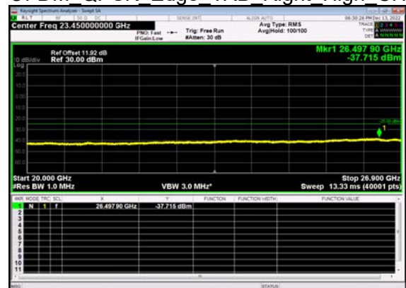
N41(60M)_DFT-s- OFDM QPSK Edge 1RB Right High CH
