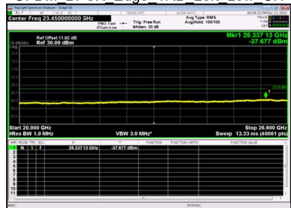
N41(60M)_DFT-s- OFDM BPSK Edge 1RB Left Low CH
