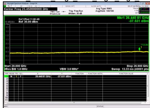
N41(40M)_DFT-s- OFDM BPSK Edge 1RB Right High CH
