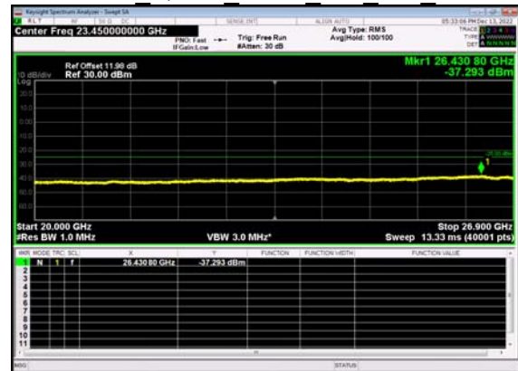
N41(40M)_DFT-s- OFDM QPSK Outer Full Mid CH
