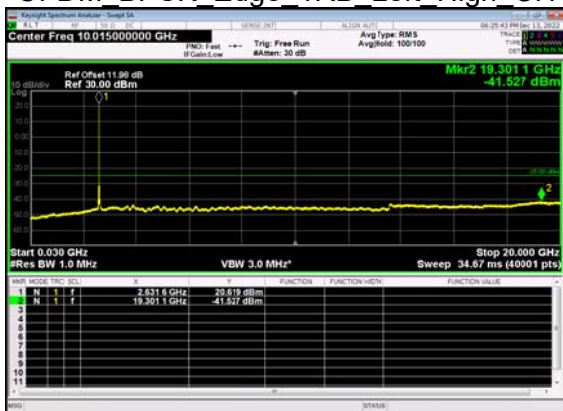
N41(60M)_DFT-s- OFDM BPSK Edge 1RB Left High CH
