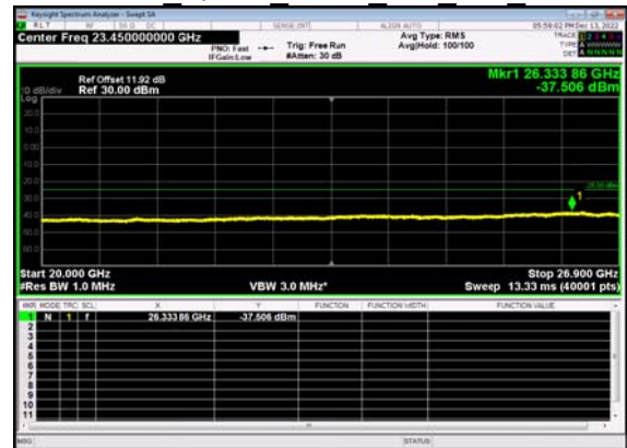
N41(50M)_DFT-s- OFDM QPSK Outer Full Mid CH
