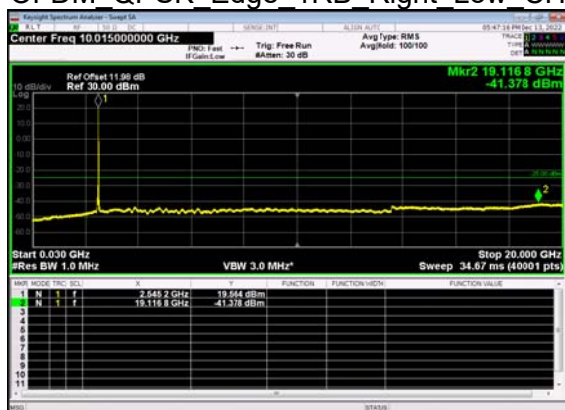
N41(50M)_DFT-s- OFDM QPSK Edge 1RB Right Low CH
