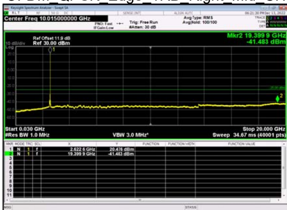
N41(60M)_DFT-s- OFDM QPSK Edge 1RB Right Mid CH
