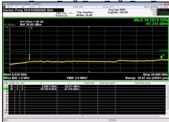
N41(60M)_DFT-s- OFDM BPSK Edge 1RB Right Low CH
