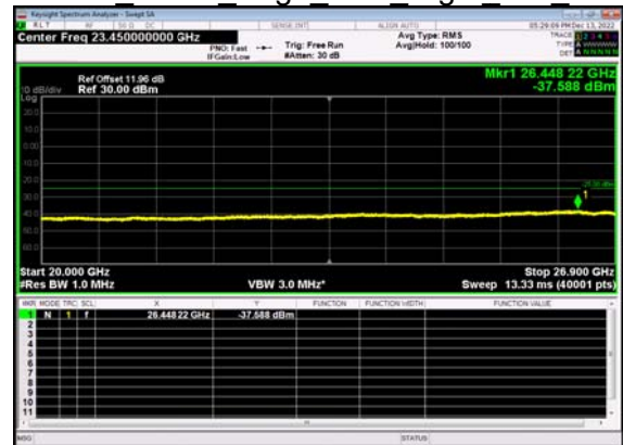
N41(40M)_DFT-s- OFDM BPSK Edge 1RB Right Mid CH
