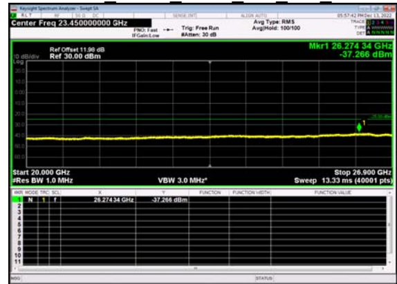
N41(50M)_DFT-s- OFDM BPSK Outer Full Mid CH
