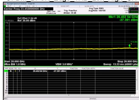
N41(40M)_DFT-s- OFDM BPSK Edge 1RB Left High CH
