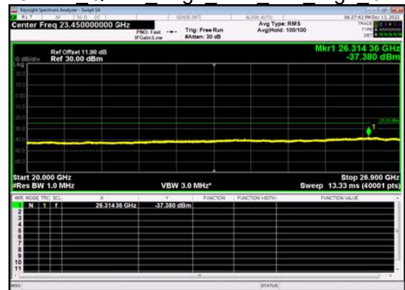
N41(60M)_DFT-s- OFDM QPSK Edge 1RB Left High CH
