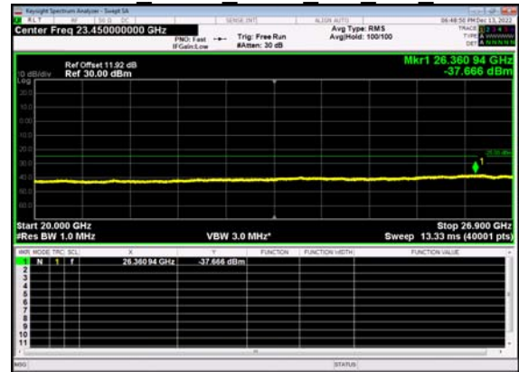
N41(80M)_DFT-s- OFDM BPSK Outer Full Mid CH
