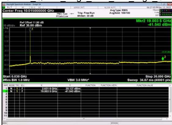
N41(60M)_DFT-s- OFDM QPSK Edge 1RB Left High CH
