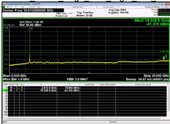
N41(40M)_DFT-s- OFDM BPSK Edge 1RB Right Mid CH
