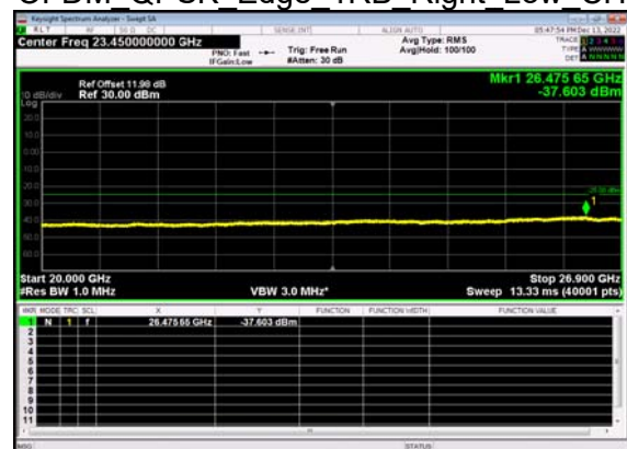
N41(50M)_DFT-s- OFDM QPSK Edge 1RB Right Low CH
