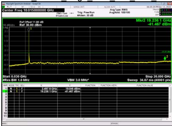
N41(80M)_DFT-s- OFDM QPSK Edge 1RB Left Low CH
