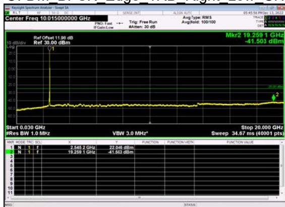
N41(50M)_DFT-s- OFDM BPSK Edge 1RB Right Low CH
