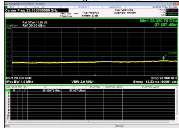
N41(80M)_DFT-s- OFDM QPSK Edge 1RB Left Mid CH
