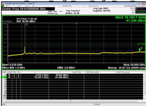
N41(80M)_DFT-s- OFDM BPSK Edge 1RB Right Low CH
