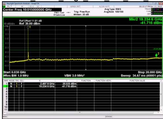
N41(60M)_DFT-s- OFDM QPSK Edge 1RB Left Low CH
