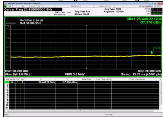
N41(40M)_DFT-s- OFDM QPSK Edge 1RB Left High CH
