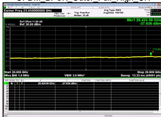
N41(40M)_DFT-s- OFDM BPSK Outer Full High CH
