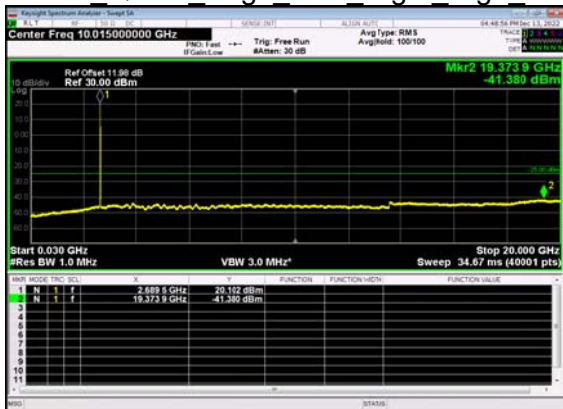
N41(20M)_DFT-s- OFDM QPSK Edge 1RB Right High CH
