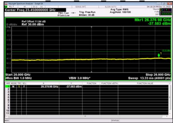
N41(15M)_DFT-s- OFDM BPSK Outer Full Mid CH
