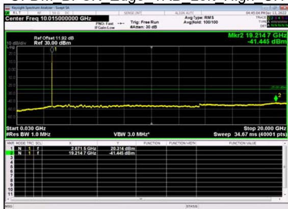
N41(20M)_DFT-s- OFDM BPSK Edge 1RB Left High CH
