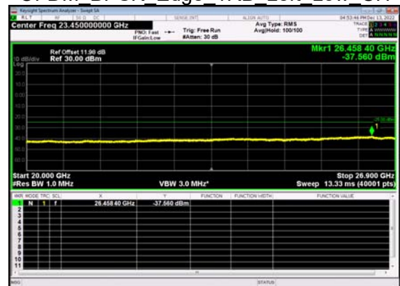
N41(30M)_DFT-s- OFDM BPSK Edge 1RB Left Low CH
