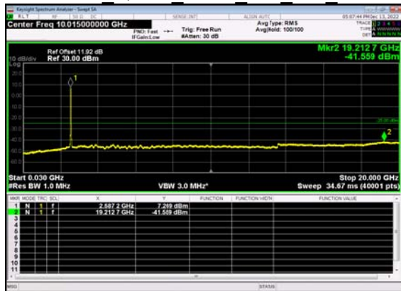
N41(30M)_DFT-s- OFDM QPSK Outer Full Mid CH
