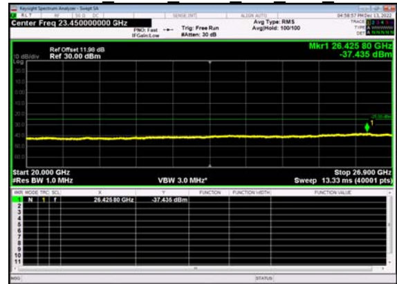
N41(30M)_DFT-s- OFDM BPSK Outer Full Low CH
