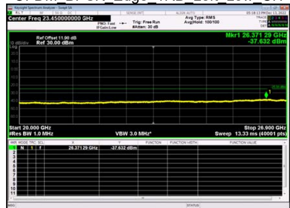
N41(40M)_DFT-s- OFDM BPSK Edge 1RB Left Low CH
