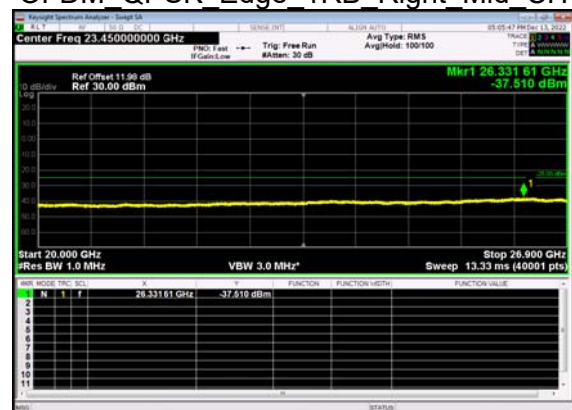
N41(30M)_DFT-s- OFDM QPSK Edge 1RB Right Mid CH
