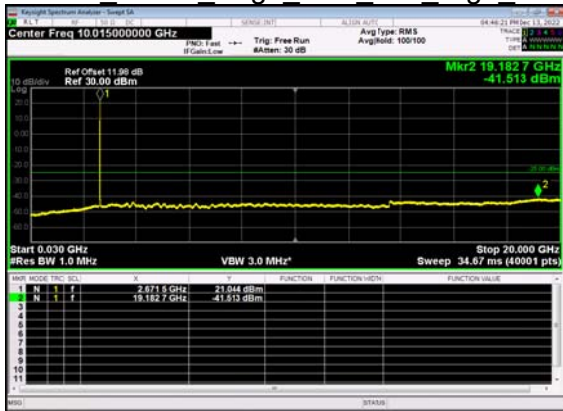
N41(20M)_DFT-s- OFDM QPSK Edge 1RB Left High CH
