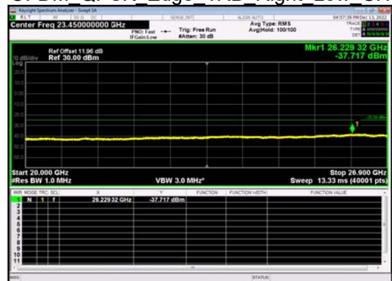
N41(30M)_DFT-s- OFDM QPSK Edge 1RB Right Low CH
