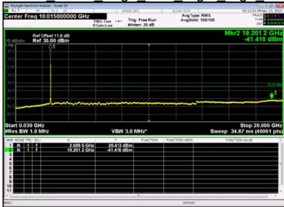
N41(30M)_DFT-s- OFDM BPSK Edge 1RB Right High CH
