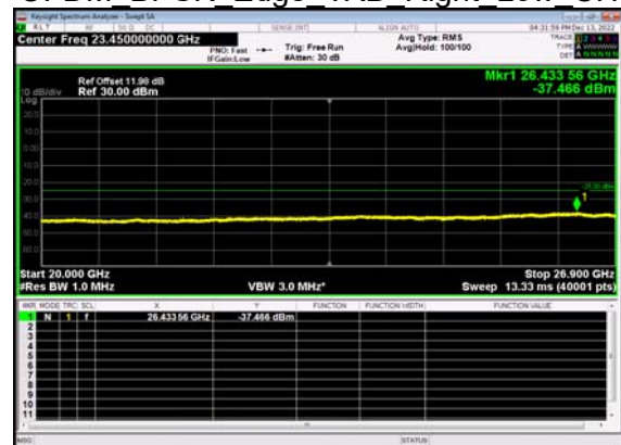
N41(20M)_DFT-s- OFDM BPSK Edge 1RB Right Low CH
