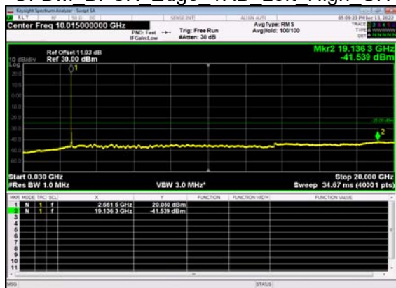
N41(30M)_DFT-s- OFDM BPSK Edge 1RB Left High CH
