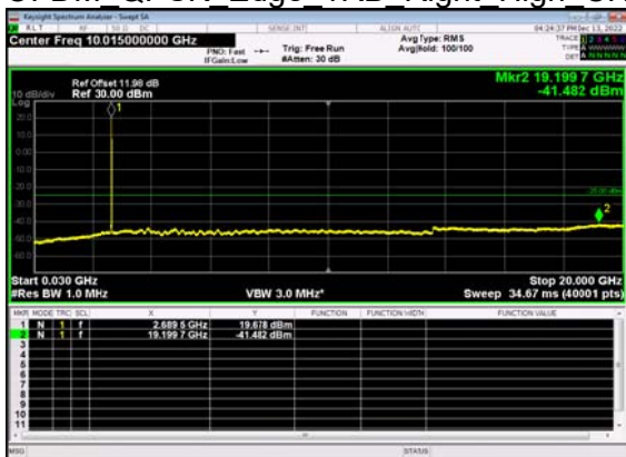
N41(15M)_DFT-s- OFDM QPSK Edge 1RB Right High CH
