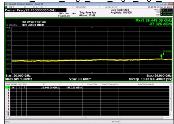
N41(30M)_DFT-s- OFDM QPSK Edge 1RB Right High CH
