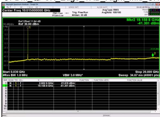
N41(20M)_DFT-s- OFDM QPSK Edge 1RB Right Mid CH
