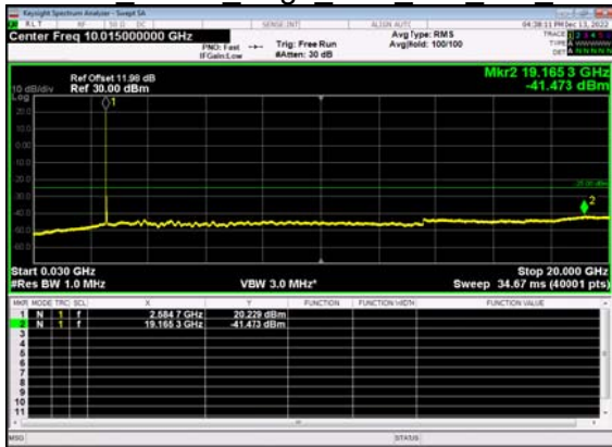
N41(20M)_DFT-s- OFDM QPSK Edge 1RB Left Mid CH
