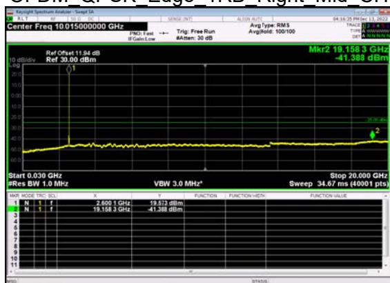
N41(15M)_DFT-s- OFDM QPSK Edge 1RB Right Mid CH
