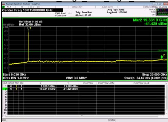
N41(30M)_DFT-s- OFDM BPSK Edge 1RB Right Low CH
