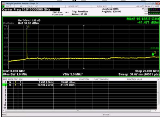
N41(40M)_DFT-s- OFDM QPSK Edge 1RB Left Low CH
