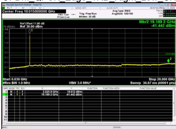
N41(30M)_DFT-s- OFDM QPSK Edge 1RB Right Low CH
