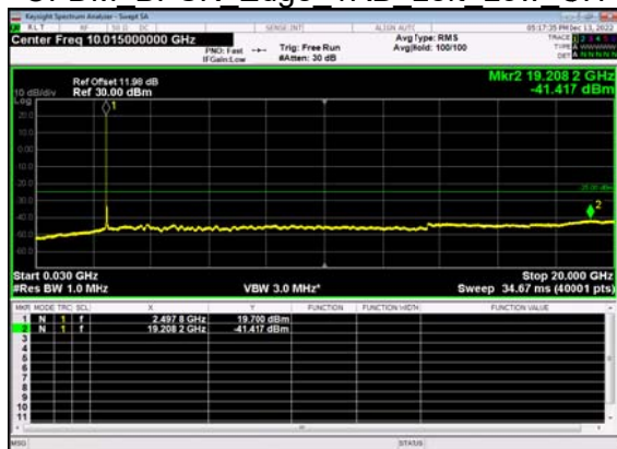
N41(40M)_DFT-s- OFDM BPSK Edge 1RB Left Low CH
