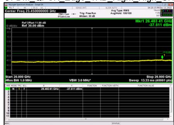
N41(15M)_DFT-s- OFDM QPSK Edge 1RB Right High CH
