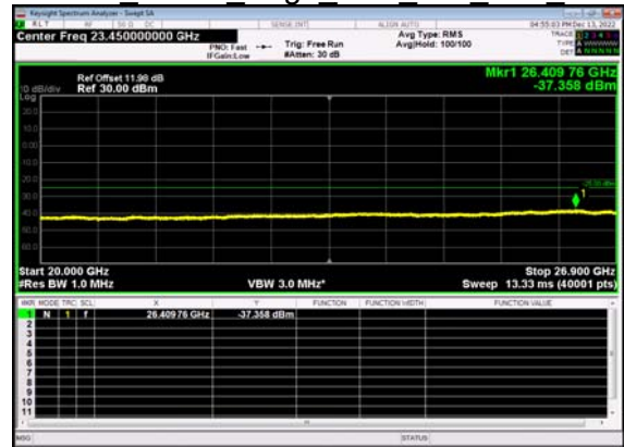
N41(30M)_DFT-s- OFDM QPSK Edge 1RB Left Low CH
