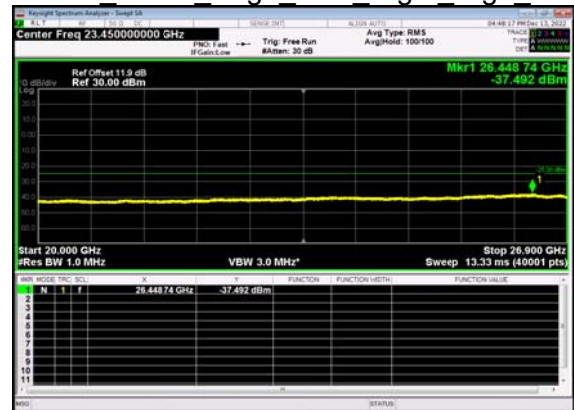
N41(20M)_DFT-s- OFDM BPSK Edge 1RB Right High CH
