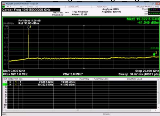
N41(15M)_DFT-s- OFDM BPSK Edge 1RB Right High CH
