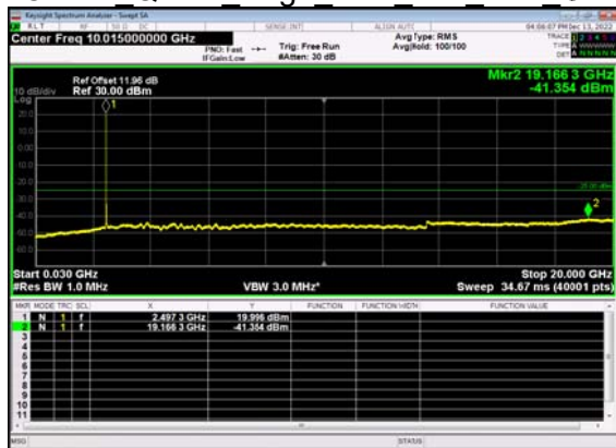
N41(15M)_DFT-s- OFDM QPSK Edge 1RB Left Low CH
