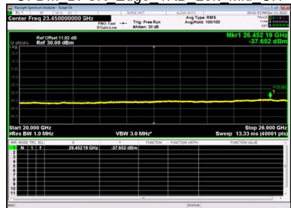
N41(30M)_DFT-s- OFDM BPSK Edge 1RB Left Mid CH
