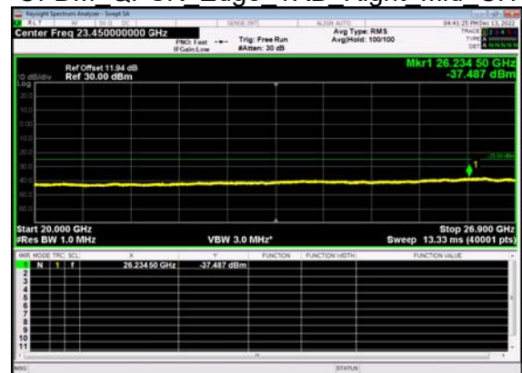
N41(20M)_DFT-s- OFDM QPSK Edge 1RB Right Mid CH
