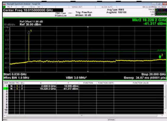
N41(15M)_DFT-s- OFDM QPSK Outer Full Low CH
