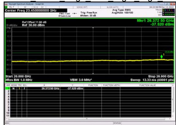
N41(15M)_DFT-s- OFDM BPSK Edge 1RB Right High CH
