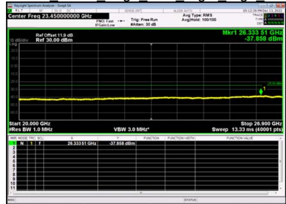
N41(30M)_DFT-s- OFDM BPSK Edge 1RB Right High CH
