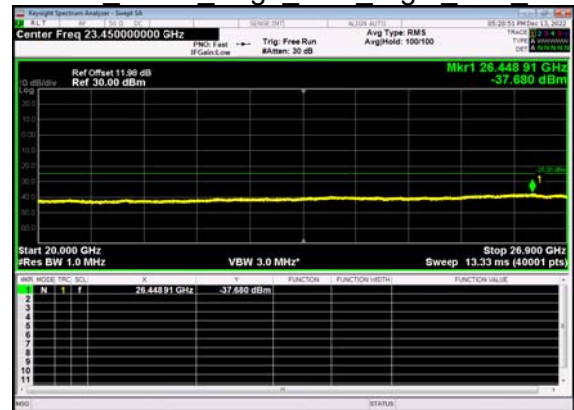
N41(40M)_DFT-s- OFDM BPSK Edge 1RB Right Low CH
