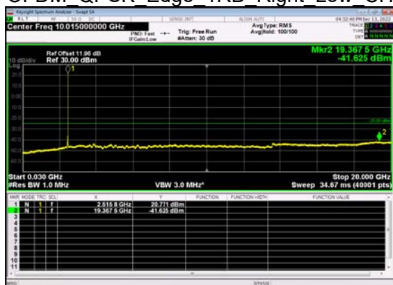
N41(20M)_DFT-s- OFDM QPSK Edge 1RB Right Low CH
