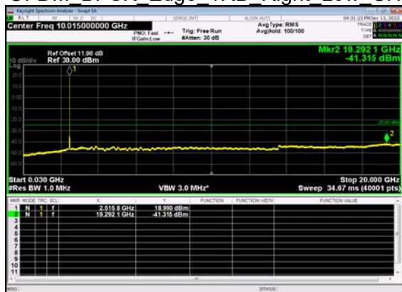
N41(20M)_DFT-s- OFDM BPSK Edge 1RB Right Low CH
