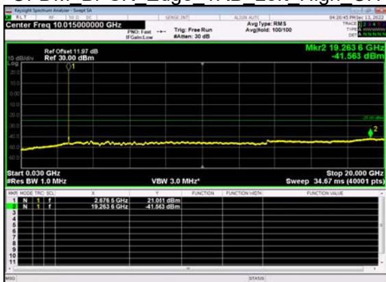
N41(15M)_DFT-s- OFDM BPSK Edge 1RB Left High CH
