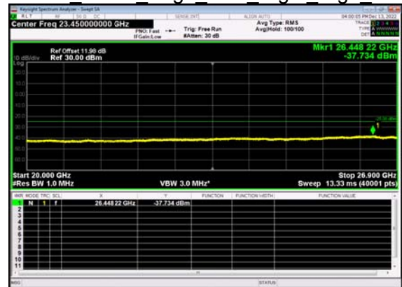
N41(10M)_DFT-s- OFDM BPSK Edge 1RB Right High CH
