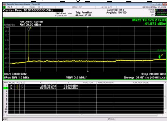
N41(20M)_DFT-s- OFDM QPSK Edge 1RB Left Low CH
