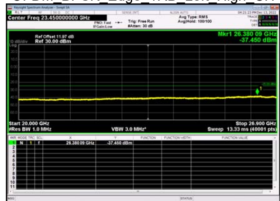
N41(15M)_DFT-s- OFDM BPSK Edge 1RB Left High CH
