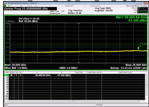
N41(30M)_DFT-s- OFDM QPSK Edge 1RB Left High CH
