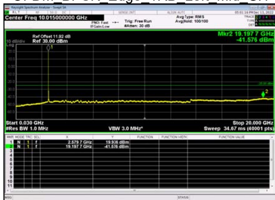
N41(30M)_DFT-s- OFDM BPSK Edge 1RB Left Mid CH
