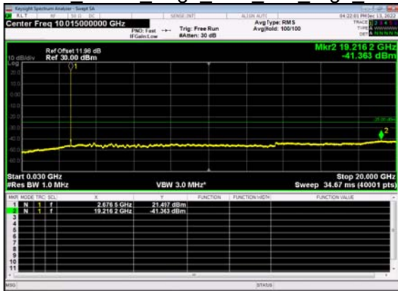
N41(15M)_DFT-s- OFDM QPSK Edge 1RB Left High CH
