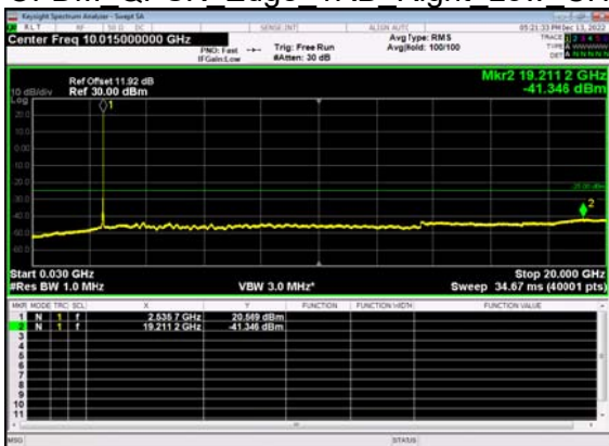
N41(40M)_DFT-s- OFDM QPSK Edge 1RB Right Low CH
