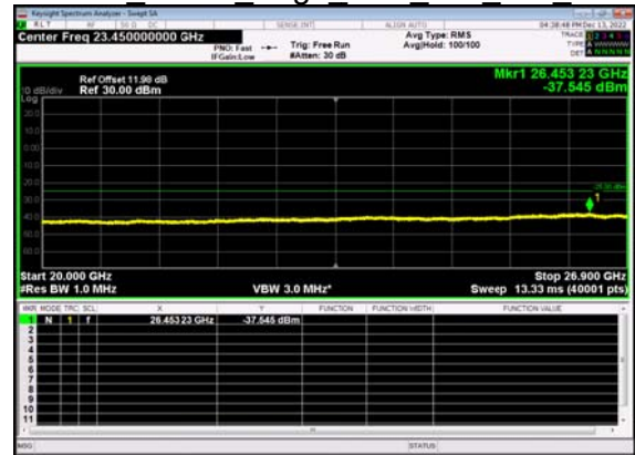
N41(20M)_DFT-s- OFDM QPSK Edge 1RB Left Mid CH
