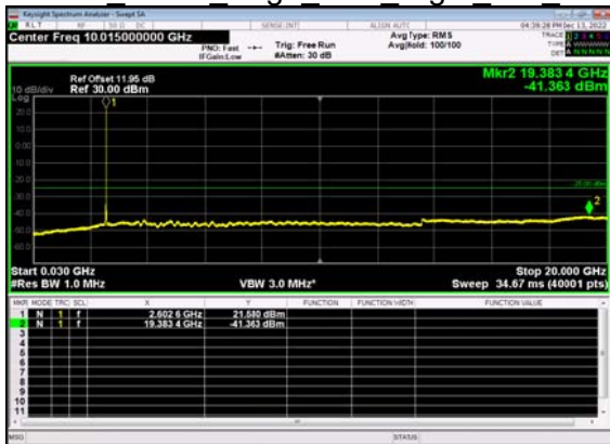
N41(20M)_DFT-s- OFDM BPSK Edge 1RB Right Mid CH
