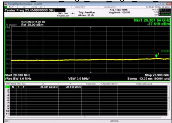
N41(30M)_DFT-s- OFDM BPSK Edge 1RB Right Low CH
