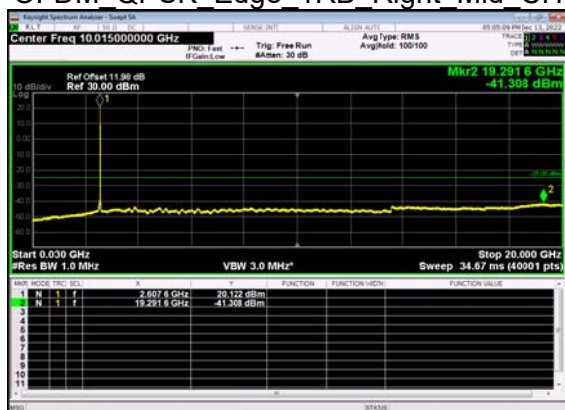
N41(30M)_DFT-s- OFDM QPSK Edge 1RB Right Mid CH
