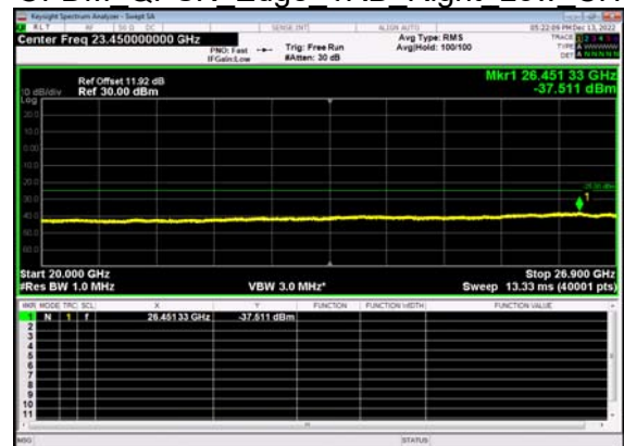
N41(40M)_DFT-s- OFDM QPSK Edge 1RB Right Low CH
