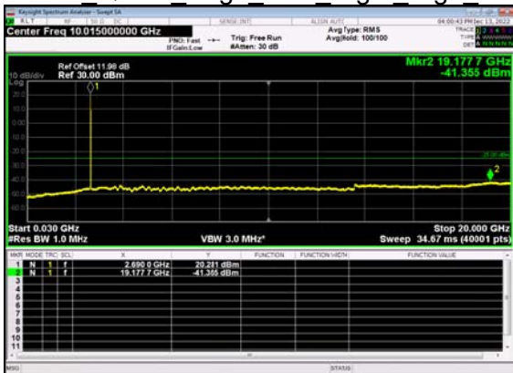
N41(10M)_DFT-s- OFDM QPSK Edge 1RB Right High CH
