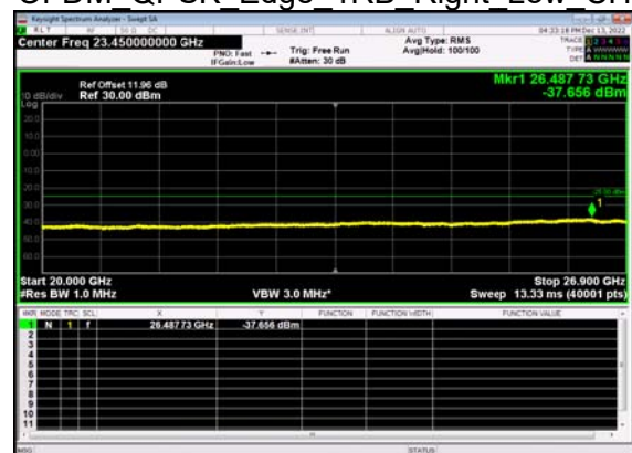
N41(20M)_DFT-s- OFDM QPSK Edge 1RB Right Low CH
