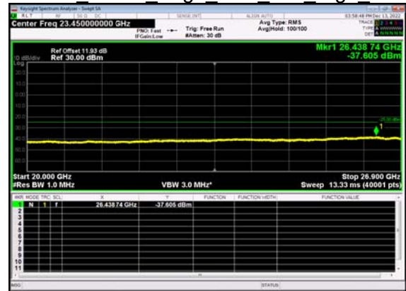
N41(10M)_DFT-s- OFDM QPSK Edge 1RB Left High CH
