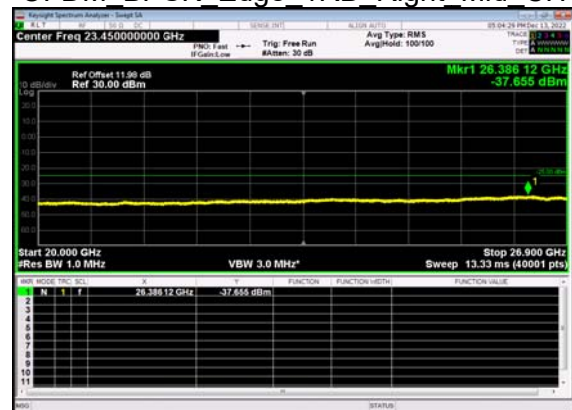
N41(30M)_DFT-s- OFDM BPSK Edge 1RB Right Mid CH
