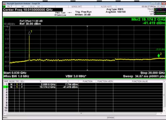
N41(30M)_DFT-s- OFDM BPSK Outer Full Mid CH
