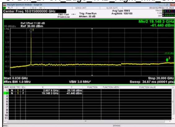
N41(30M)_DFT-s- OFDM BPSK Edge 1RB Right Mid CH
