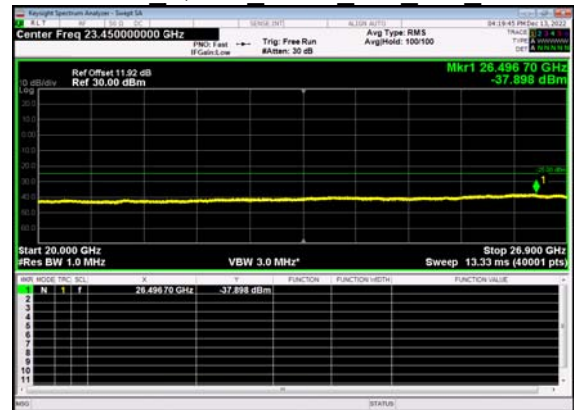
N41(15M)_DFT-s- OFDM QPSK Outer Full Mid CH
