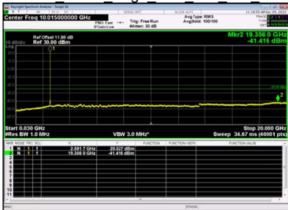
N38(10M)_DFT-s- OFDM BPSK Edge 1RB Left Mid CH
