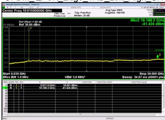
N38(10M)_DFT-s- OFDM QPSK Edge 1RB Left High CH
