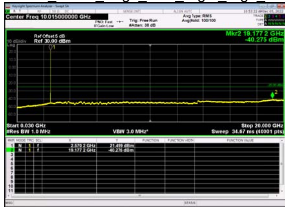
N7(10M)_DFT-s- OFDM BPSK Edge 1RB Right High CH
