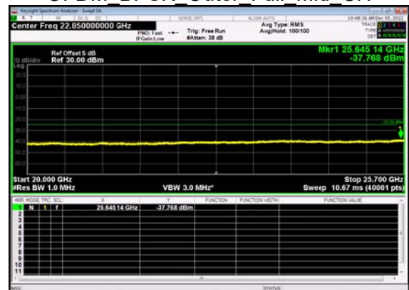
N7(10M)_DFT-s- OFDM BPSK Outer Full Mid CH
