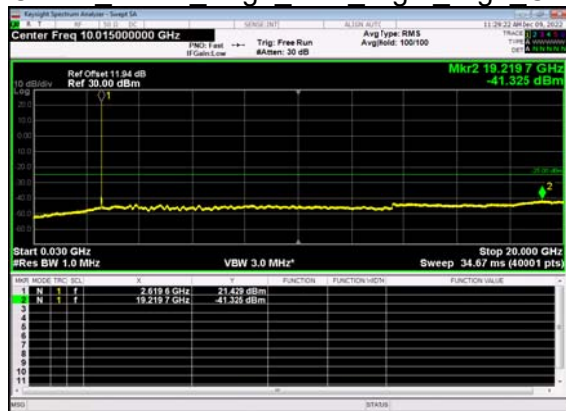
N38(10M)_DFT-s- OFDM BPSK Edge 1RB Right High CH
