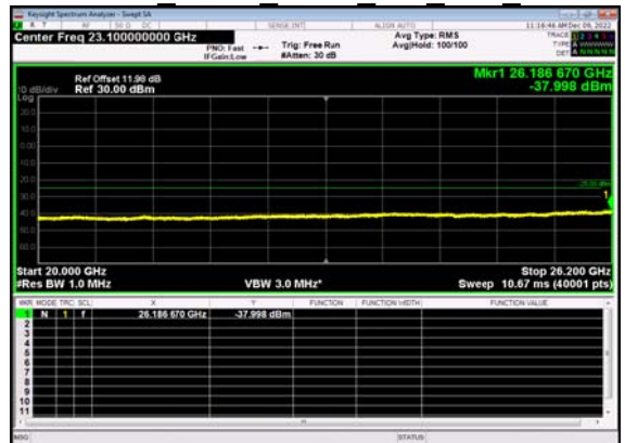
N38(10M)_DFT-s- OFDM BPSK Outer Full Low CH
