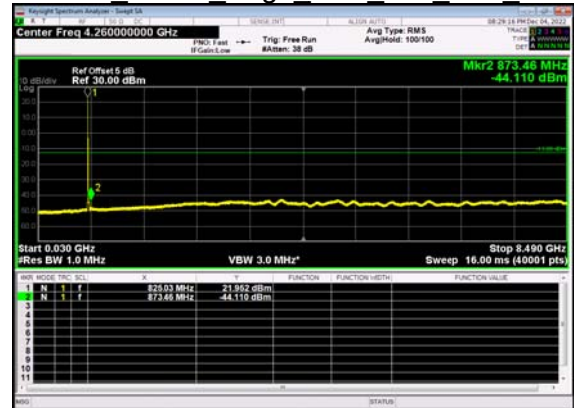
N5(10M)_DFT-s-OFDM QPSK Edge 1RB Left Low CH
