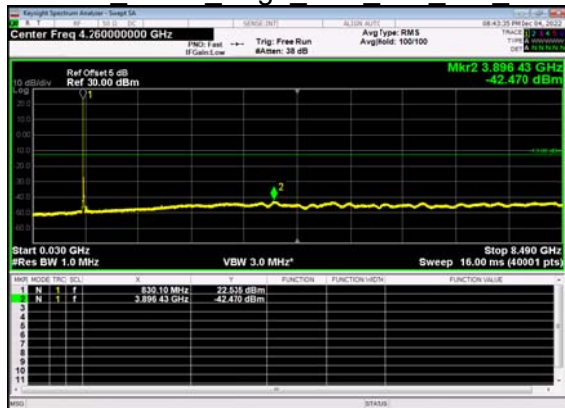
N5(15M)_DFT-s- OFDM BPSK Edge 1RB Left Mid CH
