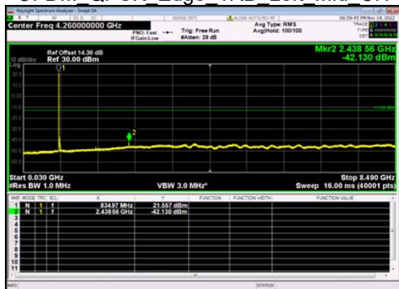
N5(5M)_DFT-s- OFDM QPSK Edge 1RB Left Mid CH
