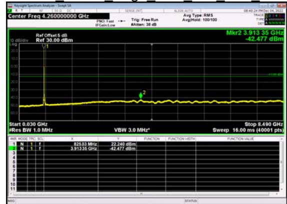
N5(15M)_DFT-s- OFDM QPSK Edge 1RB Left Low CH
