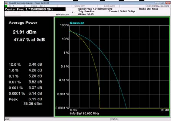
N66(10M)_DFT-s-OFDM QPSK Outer Full Low CH
