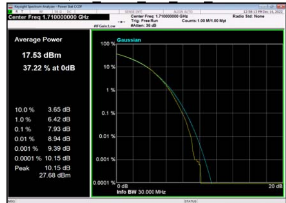
N66(30M)_CP-OFDM_16 QAM Outer Full Low CH
