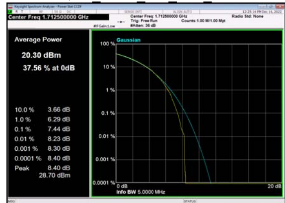
N66(5M)_CP-OFDM_16QAM Outer Full Low CH
