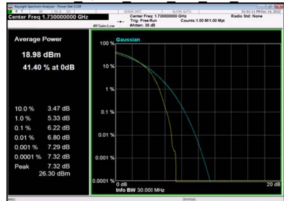
N66(30M)_DFT-s-OFDM QPSK Outer Full Mid CH
