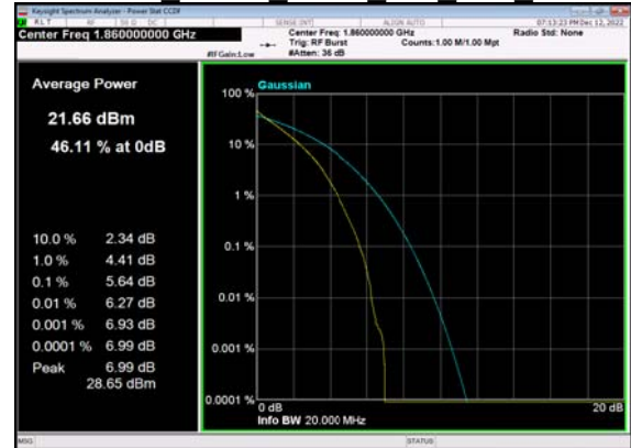
N2(20M)_DFT-s-OFDM QPSK Outer Full Low CH
