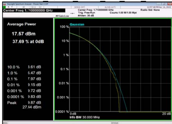
N66(30M)_CP-OFDM QPSK Outer Full Low CH
