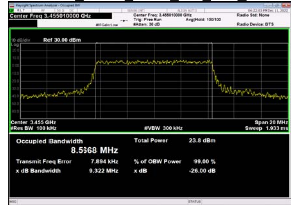
N77(10M)_CP- OFDM QPSK Outer Full Low CH
