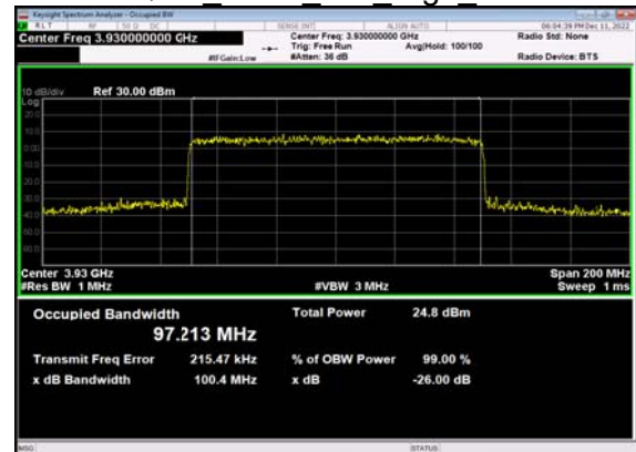
N77(100M)_CP-OFDM_64 QAM Outer Full High CH
