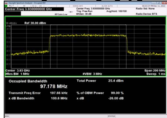
N77(100M)_CP- OFDM QPSK Outer Full High CH
