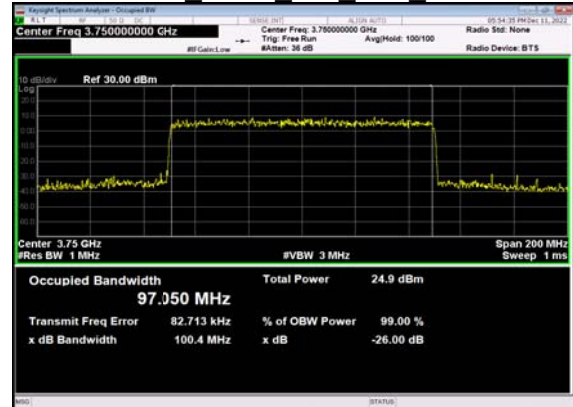
N77(100M)_CP-OFDM_64 QAM Outer Full Low CH
