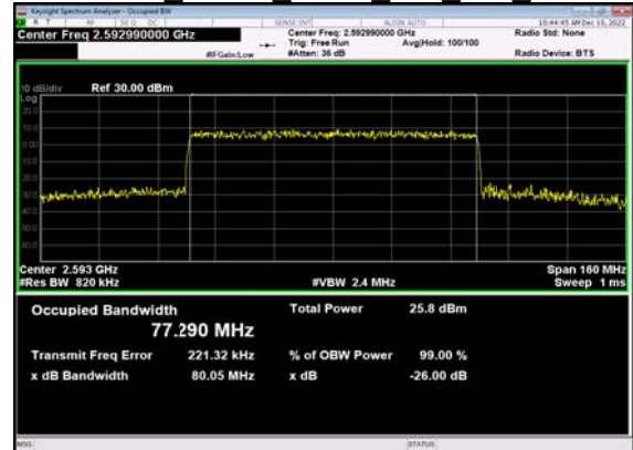
N41(80M)_CP- OFDM QPSK Outer Full Mid CH
