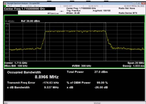
N66(10M)_DFT-s-OFDM_256 QAM Outer Full Low CH
