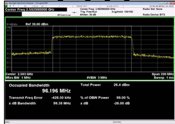
N41(100M)_DFT-s-OFDM_64 QAM Outer Full Mid CH
