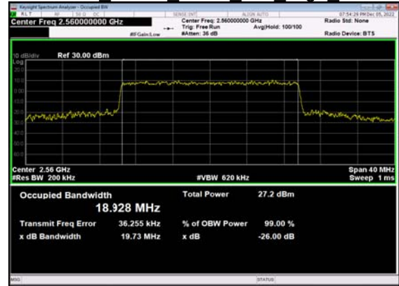
N7(20M)_CP- OFDM QPSK Outer Full High CH
