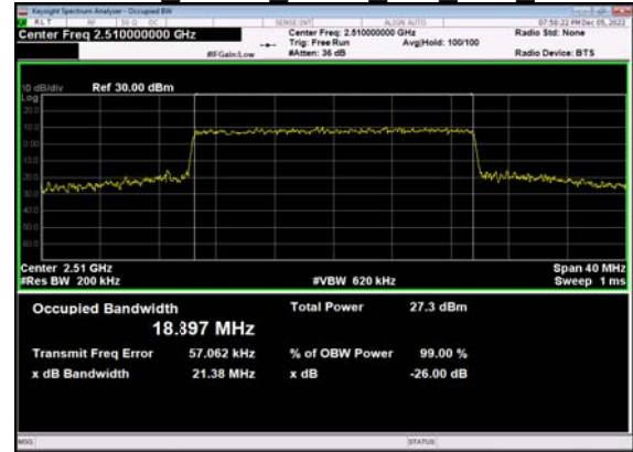
N7(20M)_CP- OFDM QPSK Outer Full Low CH
