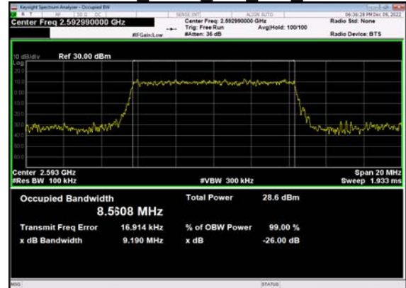
N41(10M)_DFT-s-OFDM_PI_2- BPSK Outer Full Mid CH
