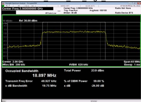
N7(20M)_CP-OFDM_256 QAM Outer Full High CH
