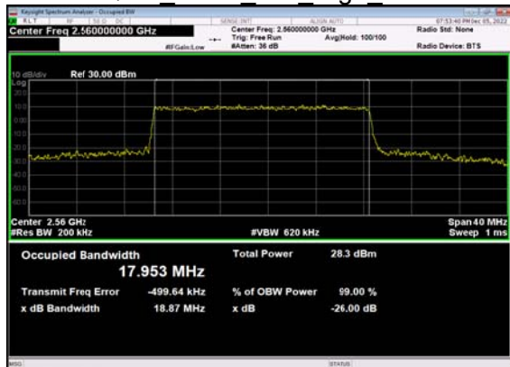
N7(20M)_DFT-s-OFDM_16 QAM Outer Full High CH
