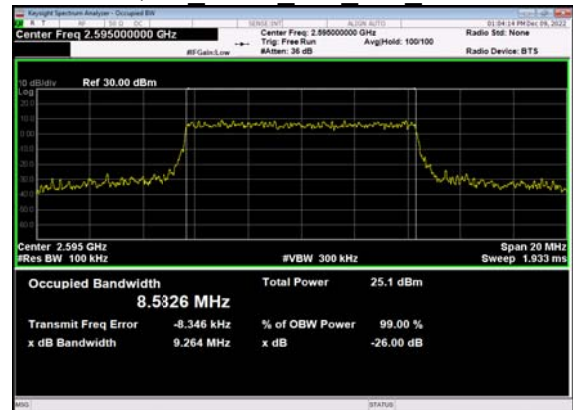
N38(10M)_CP-OFDM_16 QAM Outer Full Mid CH
