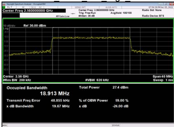
N7(20M)_CP-OFDM_16 QAM Outer Full High CH
