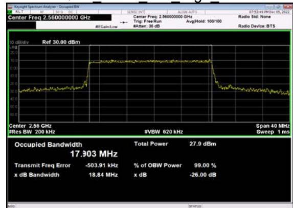
N7(20M)_DFT-s-OFDM_64 QAM Outer Full High CH
