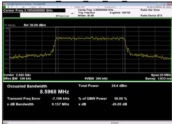
N38(10M)_CP-OFDM_64 QAM Outer Full Mid CH
