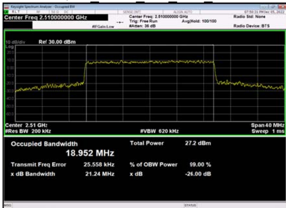
N7(20M)_CP-OFDM_16 QAM Outer Full Low CH
