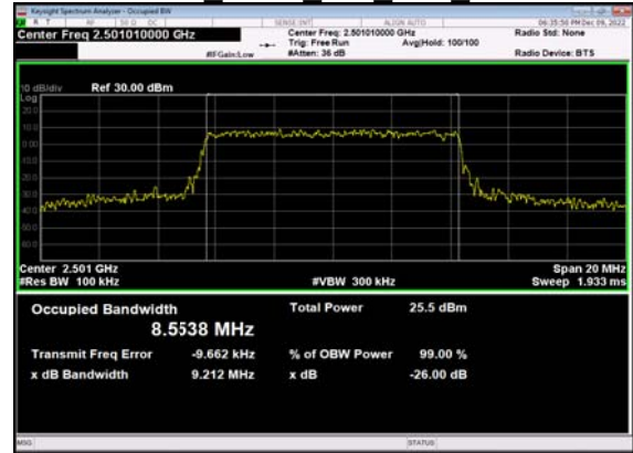
N41(10M)_CP-OFDM_64 QAM Outer Full Low CH
