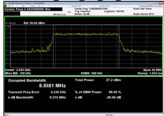
N41(10M)_DFT-s-OFDM_16 QAM Outer Full Mid CH
