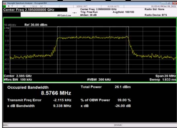
N38(10M)_DFT-s-OFDM_64 QAM Outer Full Mid CH
