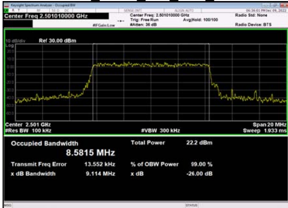
N41(10M)_CP-OFDM_256 QAM Outer Full Low CH
