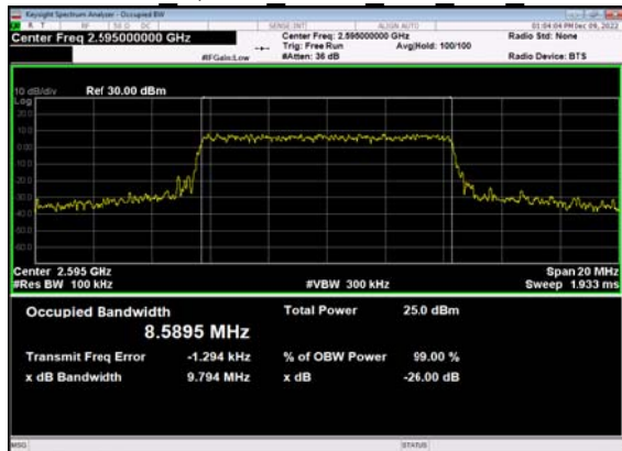
N38(10M)_CP- OFDM QPSK Outer Full Mid CH
