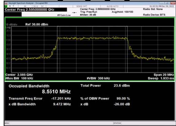
N38(10M)_DFT-s-OFDM_256 QAM Outer Full Mid CH
