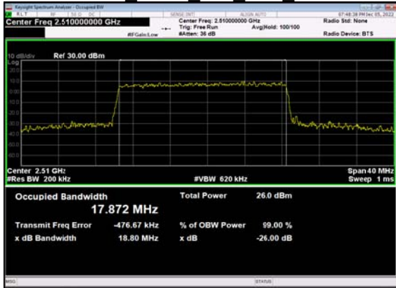
N7(20M)_DFT-s-OFDM_256 QAM Outer Full Low CH
