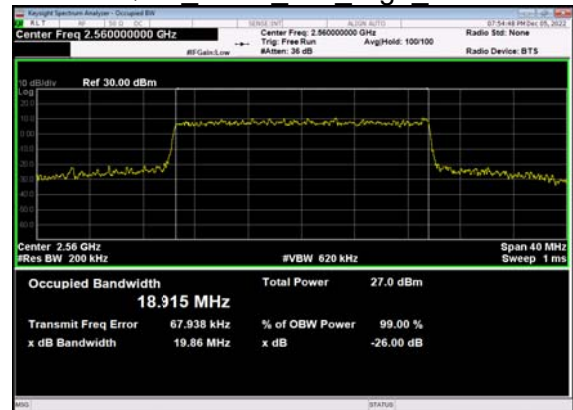
N7(20M)_CP-OFDM_64 QAM Outer Full High CH
