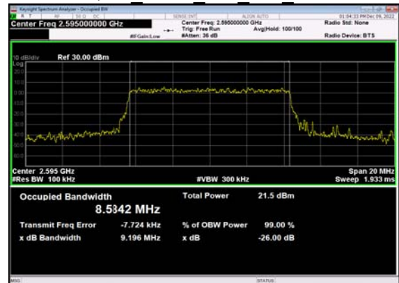
N38(10M)_CP-OFDM_256 QAM Outer Full Mid CH
