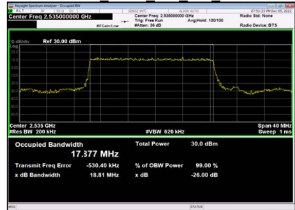
N7(20M)_DFT-s-OFDM_PI_2- BPSK Outer Full Mid CH
