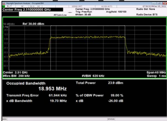
N7(20M)_CP-OFDM_256 QAM Outer Full Low CH
