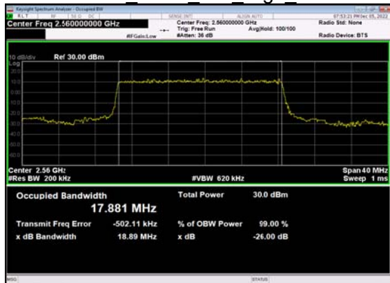
N7(20M)_DFT-s-OFDM_PI_2- BPSK Outer Full High CH
