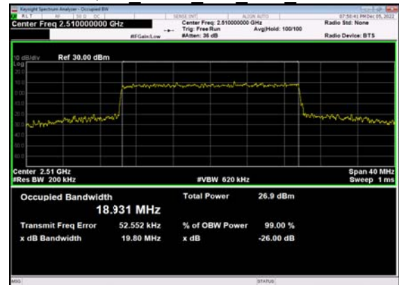
N7(20M)_CP-OFDM_64 QAM Outer Full Low CH
