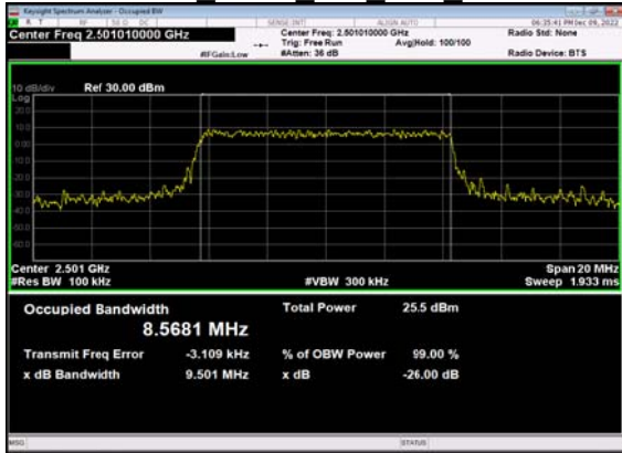
N41(10M)_CP-OFDM_16 QAM Outer Full Low CH
