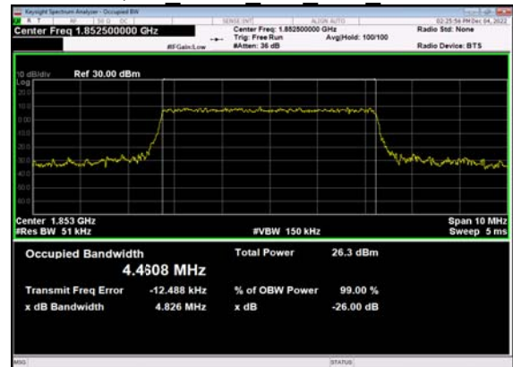
N2(5M)_CP-OFDM_64 QAM Outer Full Low CH
