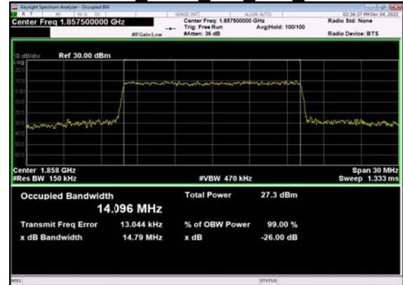
N2(15M)_CP-OFDM_ QPSK Outer Full Low CH
