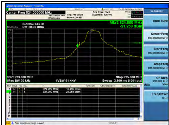
Band26Part22 / 1.4MHz / Low CH / QPSK / 1 RB
