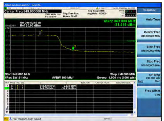
Band26Part22 / 5MHz / High CH / QPSK / FULL RB
