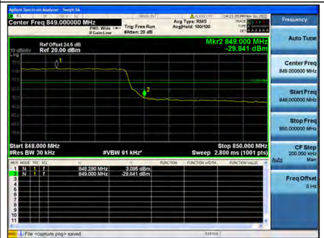
Band26Part22 / 3MHz / High CH / QPSK / FULL RB
