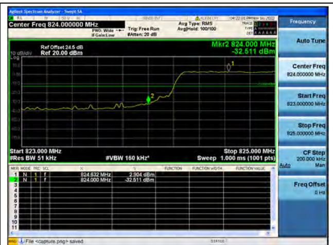
Band26Part22 / 5MHz / Low CH / QPSK / FULL RB
