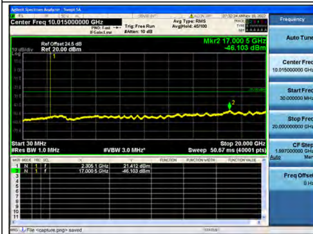
Band30-30M-20G / 5MHz / Low CH / 64QAM
