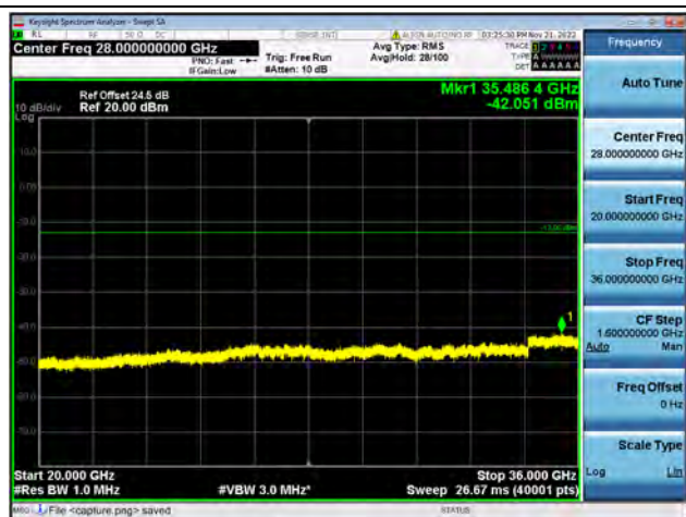
Band42-20G-36G / 20MHz / Low CH / 64QAM
