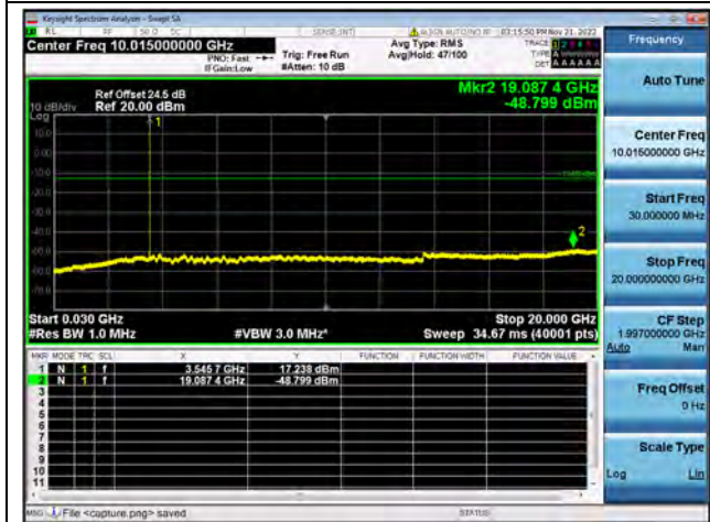
Band42-30M-20G / 5MHz / High CH / 16QAM
