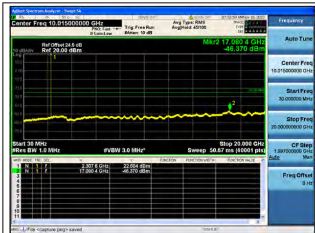
Band30-30M-20G / 5MHz / Mid CH / QPSK
