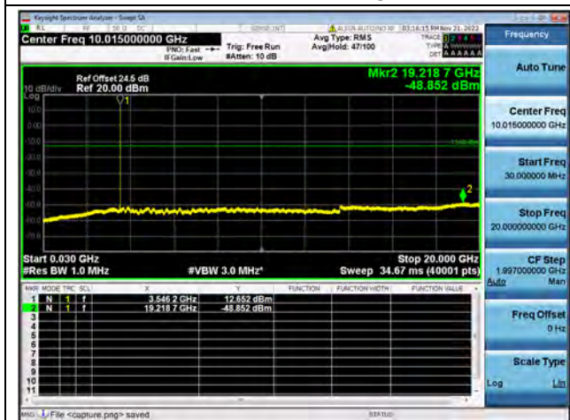
Band42-30M-20G / 5MHz / High CH / 64QAM
