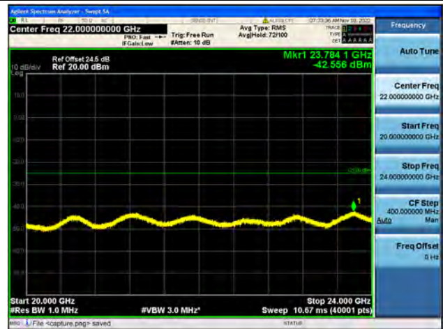
Band30-20G-24G / 5MHz / Mid CH / 16QAM
