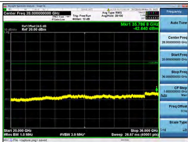
Band42-20G-36G / 20MHz / Low CH / 16QAM
