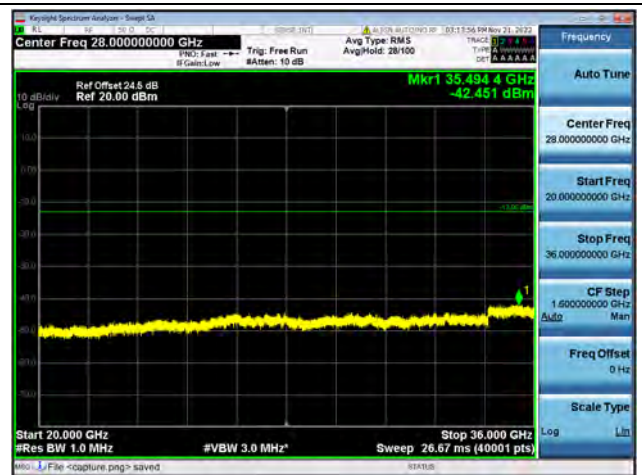
Band42-20G-36G / 5MHz / Low CH / 64QAM
