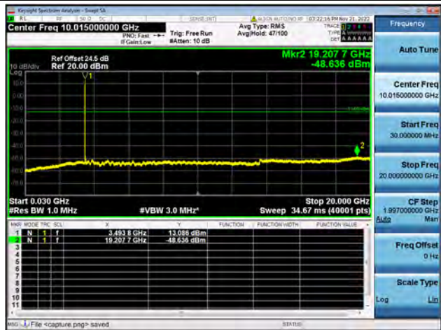
Band42-30M-20G / 15MHz / Mid CH / 16QAM
