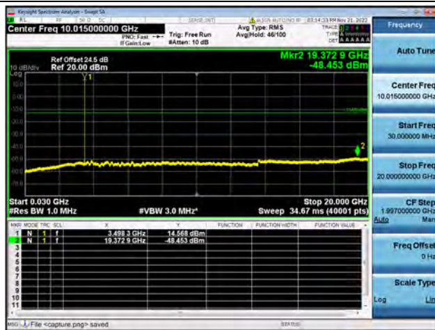
Band42-30M-20G / 5MHz / Mid CH / 16QAM
