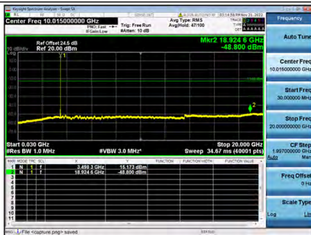
Band42-30M-20G / 5MHz / Mid CH / 64QAM
