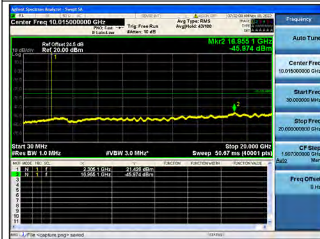
Band30-30M-20G / 5MHz / Low CH / 16QAM
