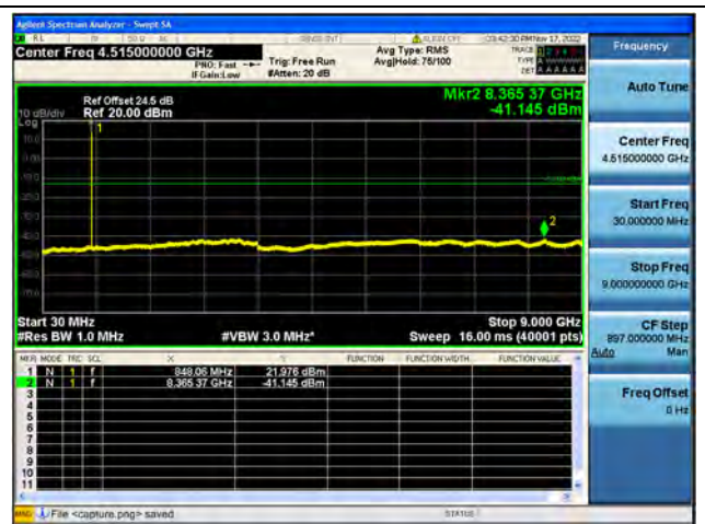
Band26Part22 / 1.4MHz / High CH / 16QAM
