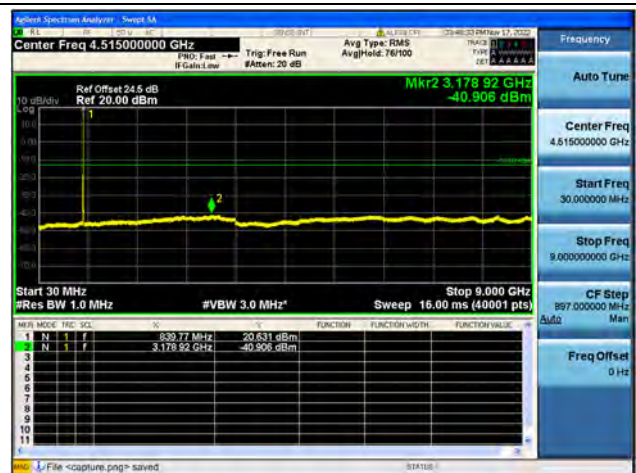
Band26Part22 / 10MHz / High CH / 64QAM
