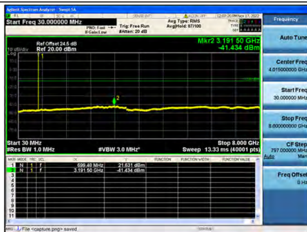
Band12 / 3MHz / Low CH / 16QAM
