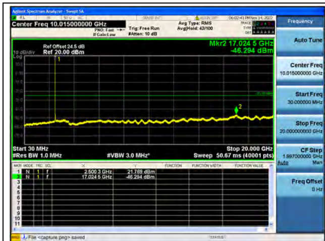
Band7-30M-20G / 10MHz / Low CH / QPSK
