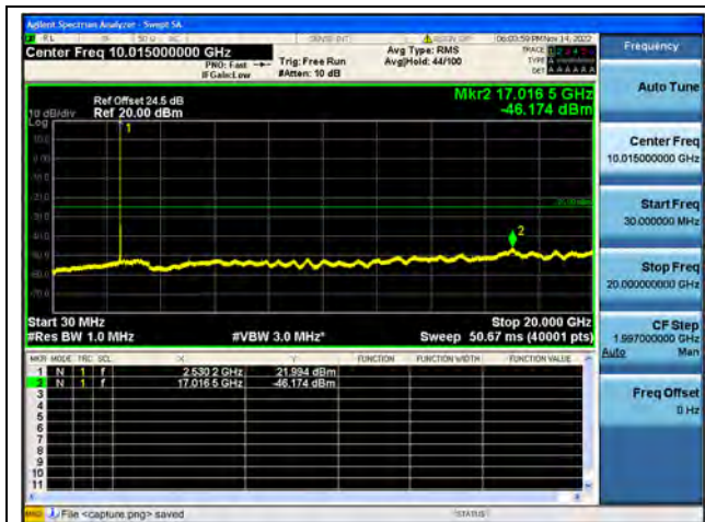
Band7-30M-20G / 10MHz / Mid CH / QPSK
