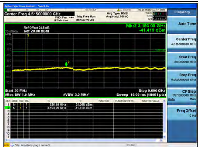
Band26Part22 / 1.4MHz / Mid CH / 64QAM
