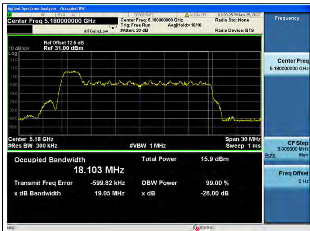
(Channel 36, 5180MHz, 802.11ax (HEW20) RU26)
