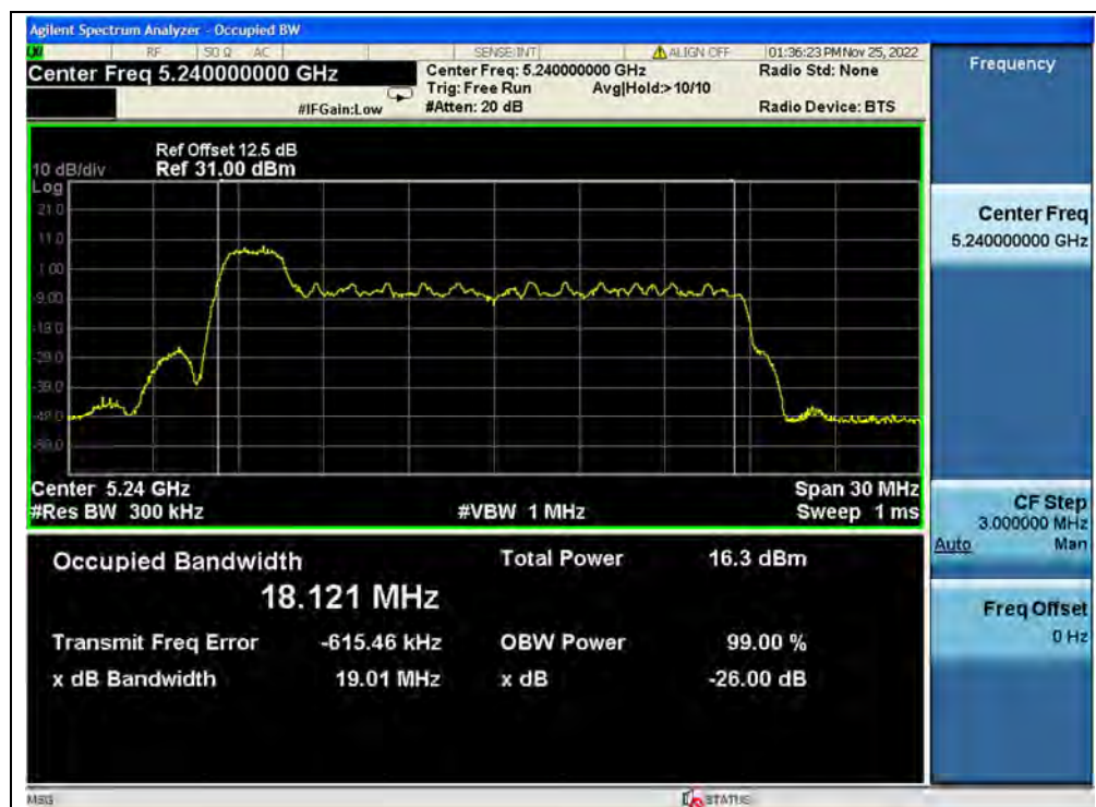
(Channel 48, 5240MHz, 802.11ax (HEW20) RU26)
