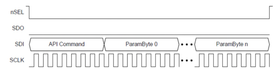
Figure 4. SPI Write Command
