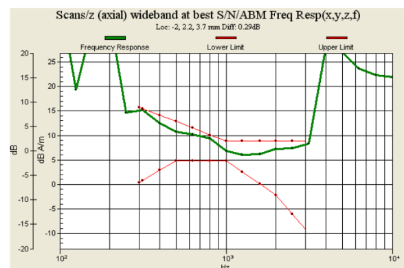
Fig. 9.4 GSM850 Ch189 (Battery 2)
