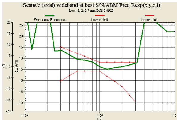
Fig. 9.1 GSM850 Ch189 (Battery 1)
