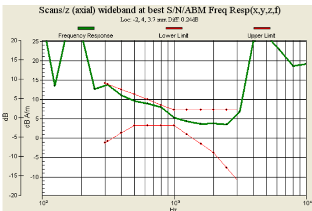
Fig. 9.9 WCDMA Band V Ch4182 (Battery 1)
