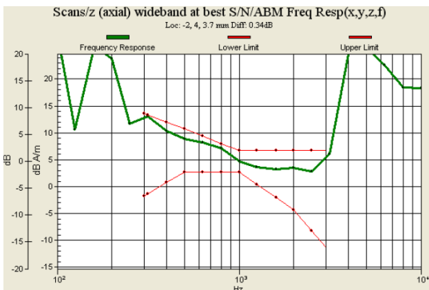
Fig. 9.11 CDMA Band V Ch4233 (Battery 1)
