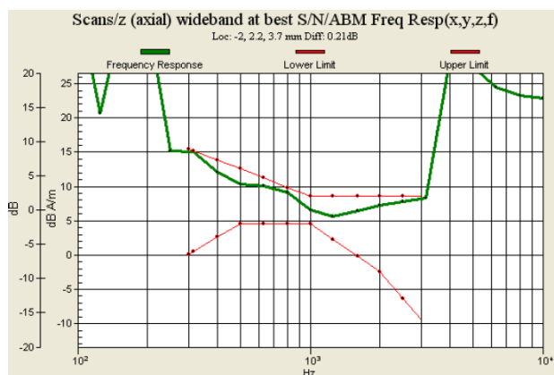
Fig. 9.5 GSM1900 Ch661 (Battery 1)
