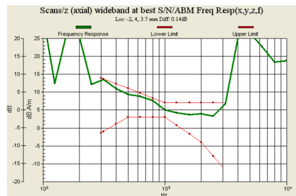
Fig. 9.15 WCDMA Band II Ch9538 (Battery 1)
