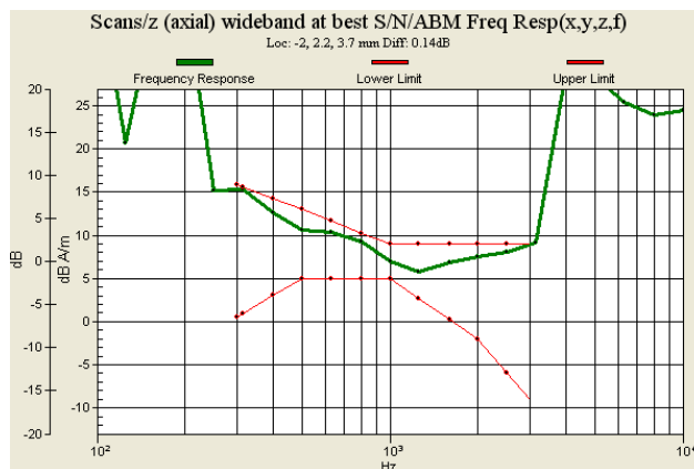
Fig. 9.3 GSM850 Ch251 (Battery 1)
