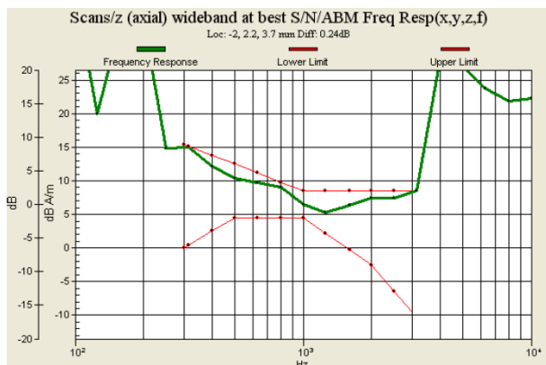
Fig. 9.7 GSM1900 Ch810 (Battery 1)
