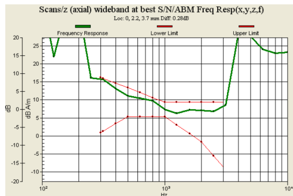
Fig. 9.8 GSM1900 Ch512 (Battery 2)
