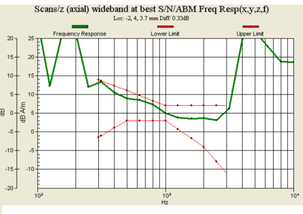
Fig. 9.12 WCDMA Band V Ch4233 (Battery 2)
