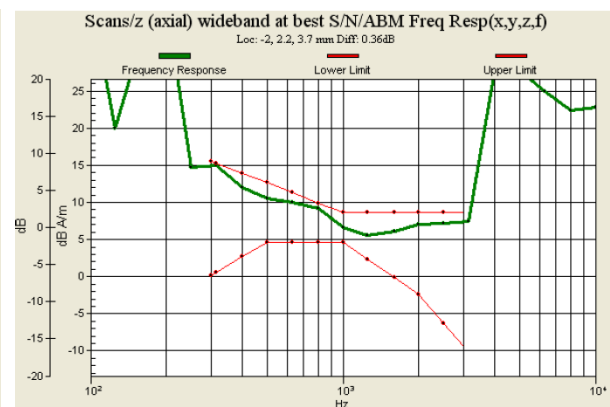
Fig. 9.2 GSM850 Ch128 (Battery 1)
