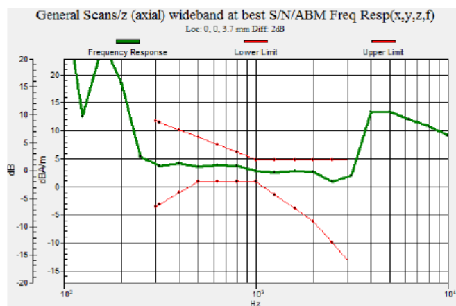
Fig 9.5 GSM1900 Ch661
