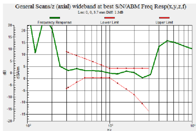
Fig 9.3 GSM850 Ch251
