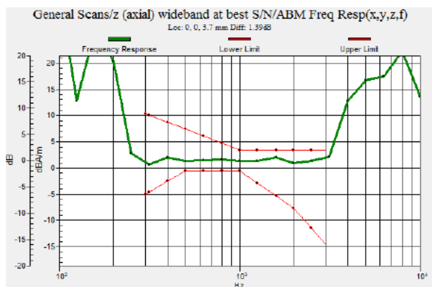
Fig 9.1 GSM850 Ch128
