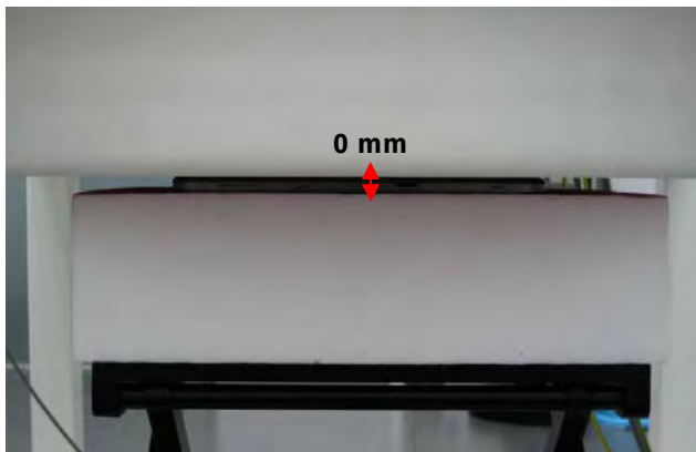
Fig.3 EUT Lap-held mode to flat phantom
