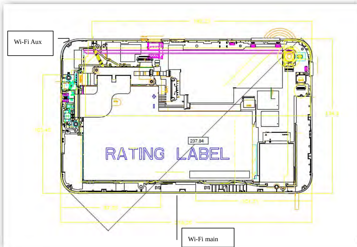
Fig.9 Antenna position of EUT
