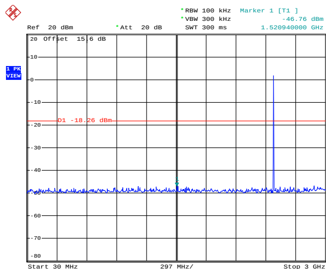
2Mbps CSE Plot on Ch 78 between 30MHz ~ 3 GHz
