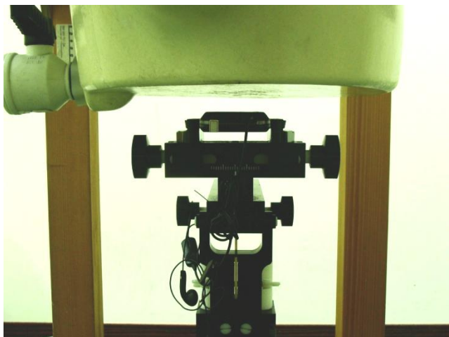
Bottom of the DUT with Phantom 1.5 cm Gap (DUT Slide Off)
