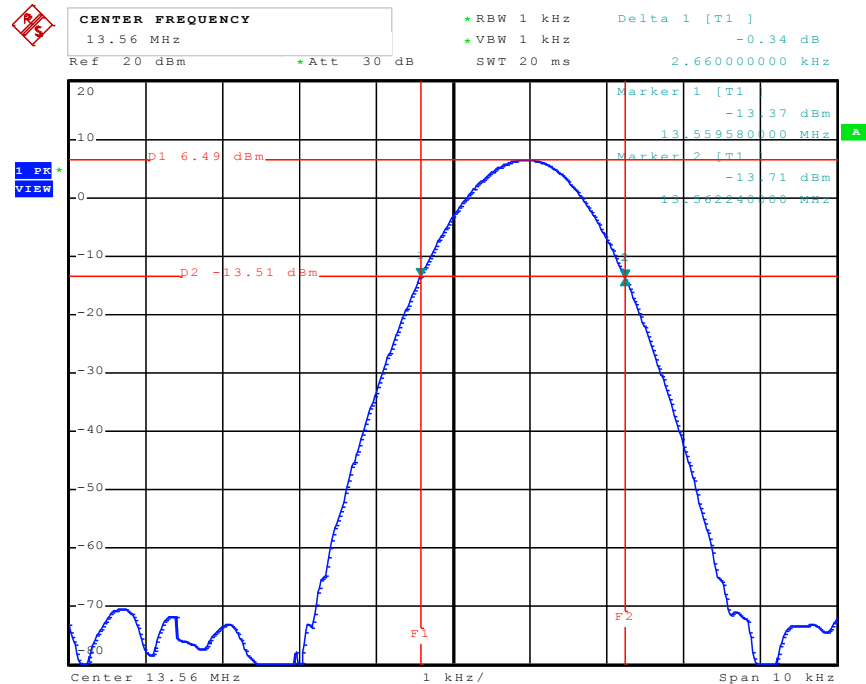
20 dB Bandwidth Plot on 13.56 MHz
