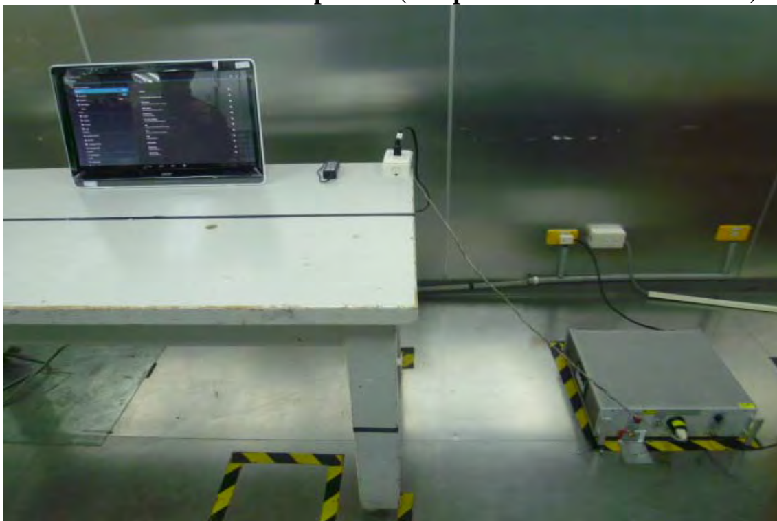
Conducted Emission Set up Photo(Adapter Model No.: DA-40C19)
