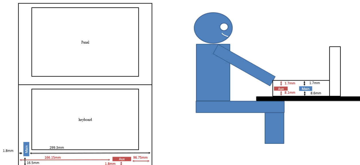
Photograph 5. Antenna position of EUT
