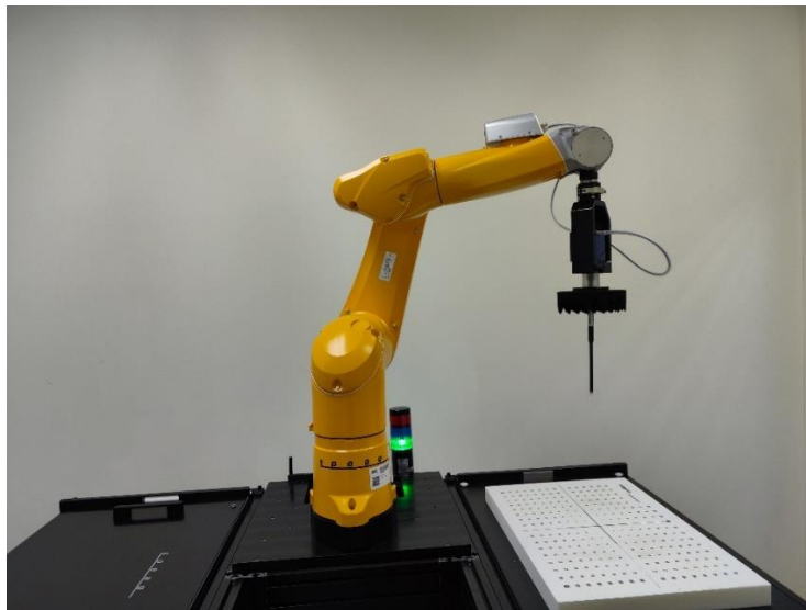
Fig.2 Photograph of the mmWave measurement system
