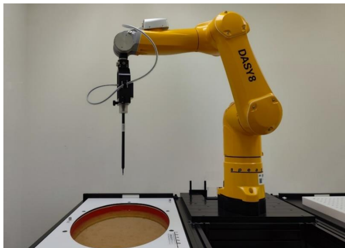
Fig.1 Photograph of the SAR measurement system
