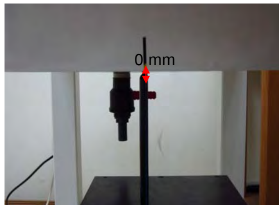
Fig.4 EUT Primary Portrait mode to flat phantom
