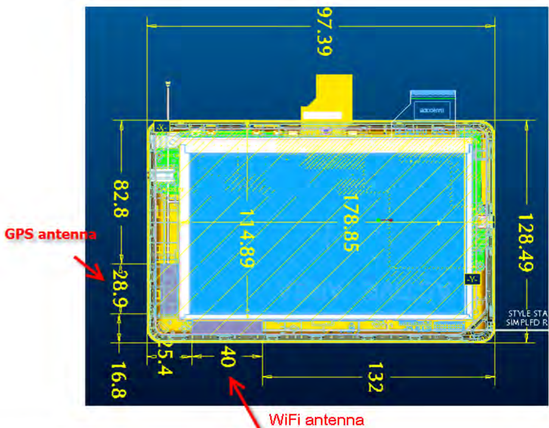
Fig.8 Antenna position of EUT
