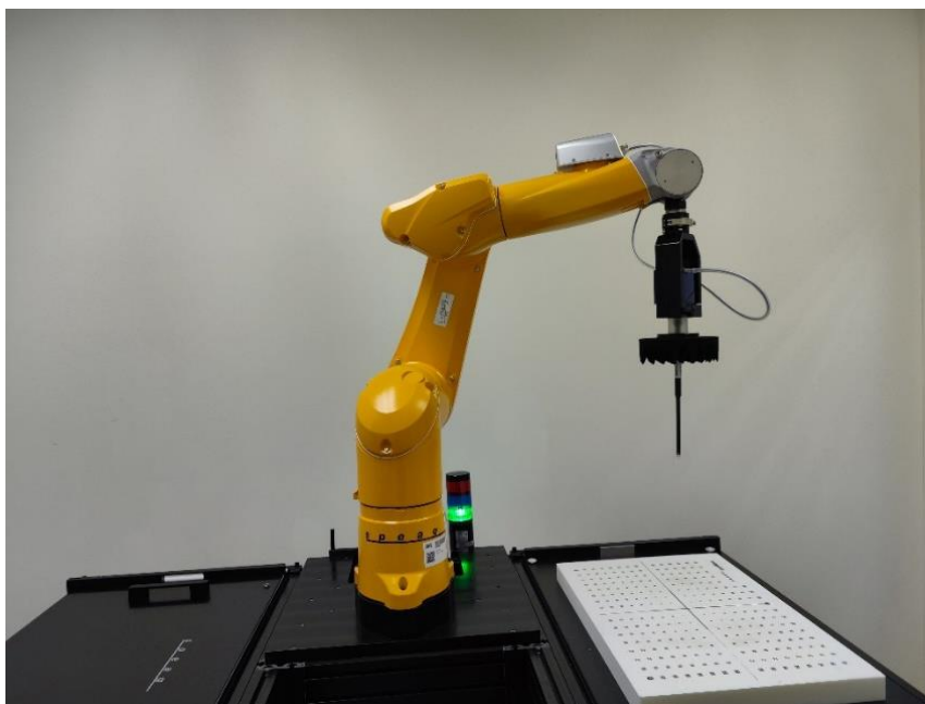
Fig.2 Photograph of the mmW measurement system
