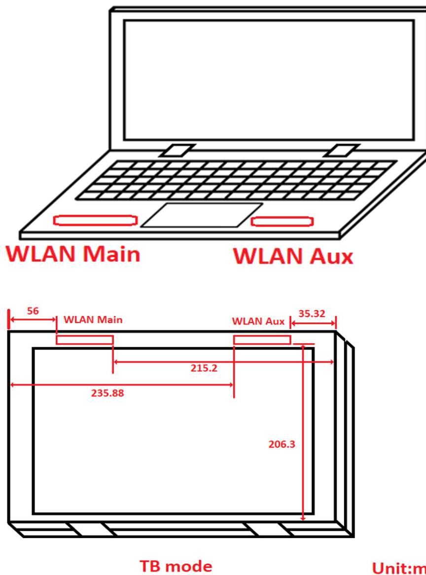
Photograph 17. Antenna position of EUT
