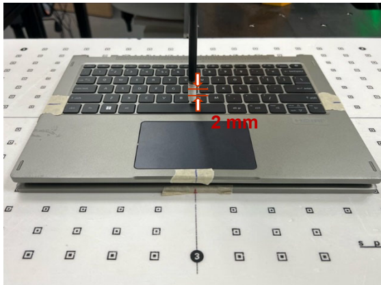
Photograph 13. PD, Front Surface, 2mm
