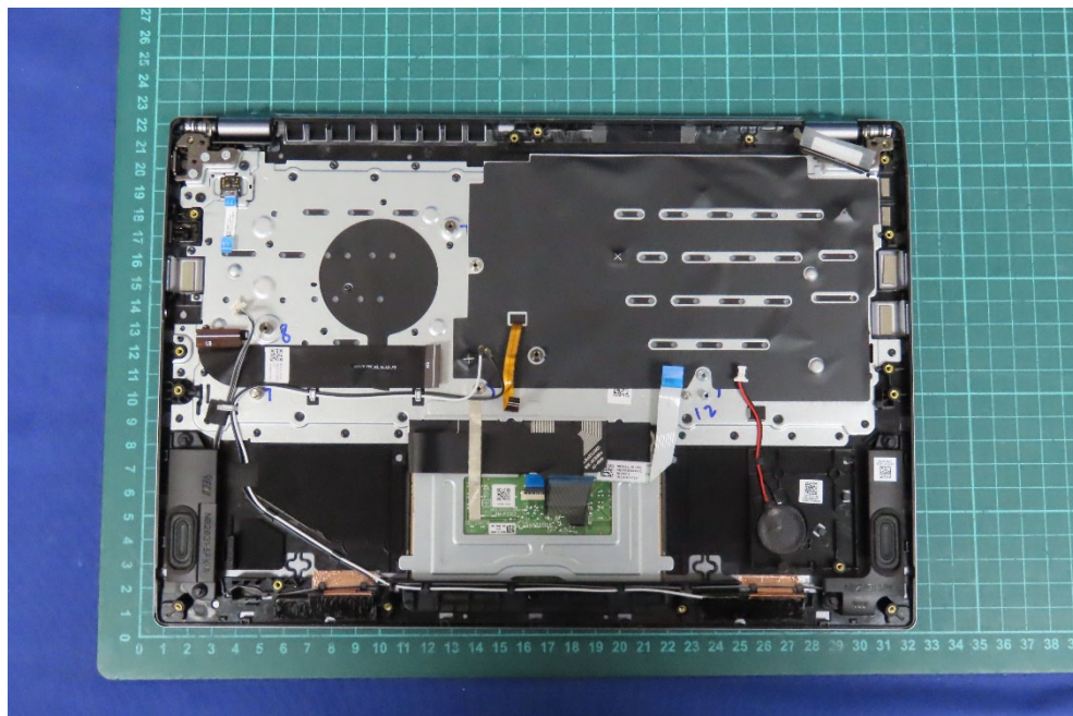
(25) EUT Photo
