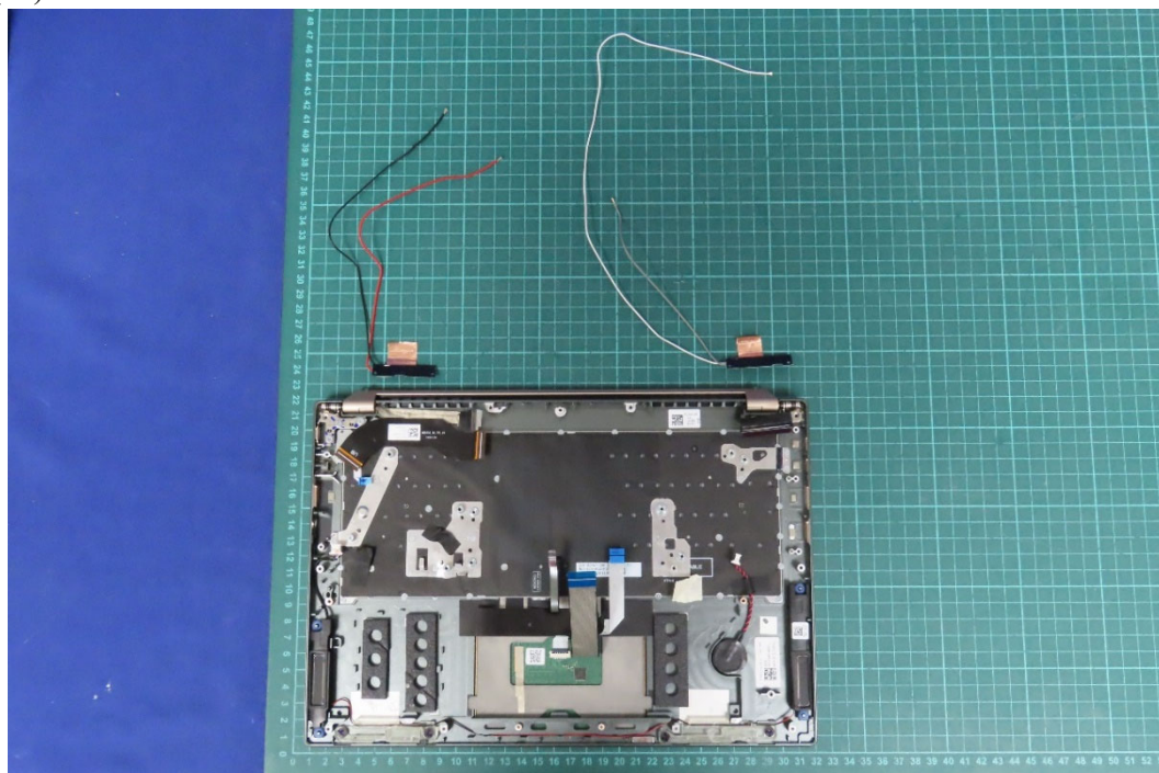
(28) EUT Photo
