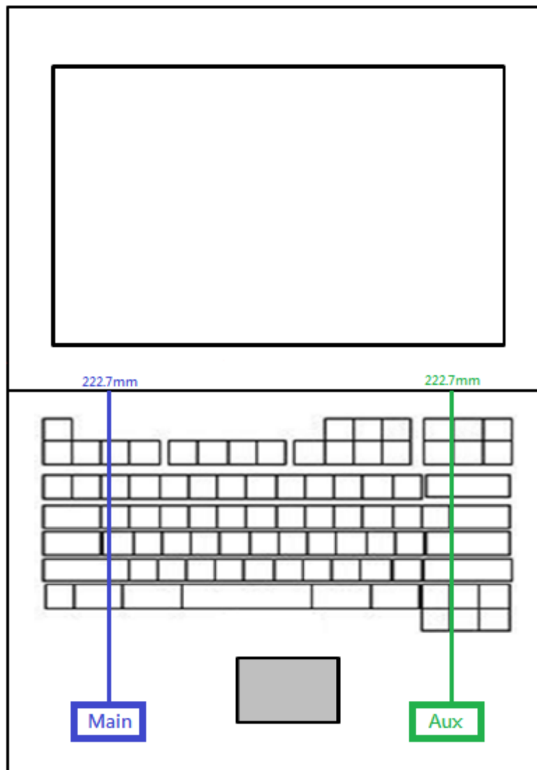
Photograph 7. Antenna position of EUT
