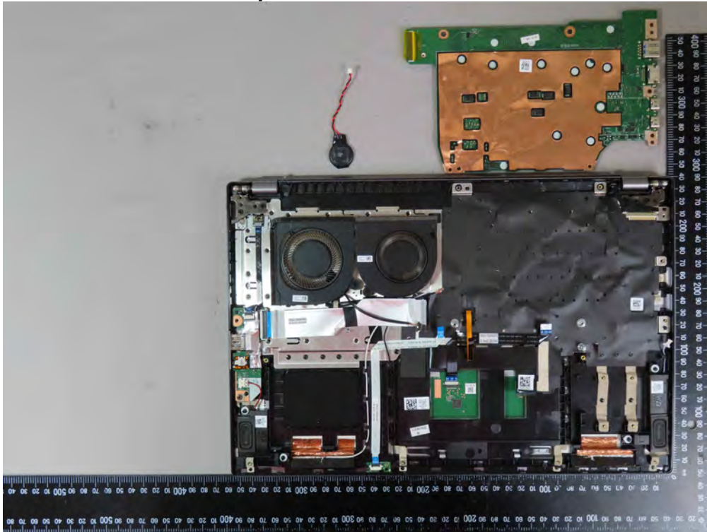
Open View of EUT – 7
