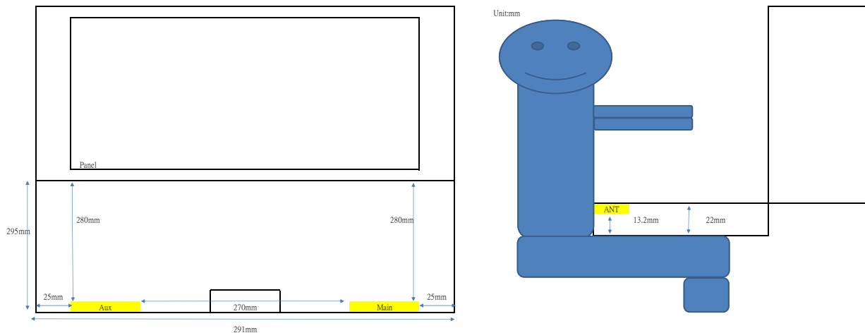
Photograph 7. Antenna position of EUT
