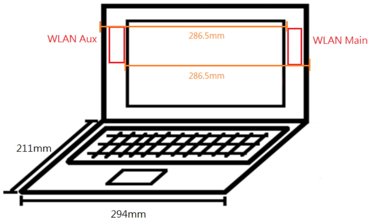
Photograph 19. Antenna position of EUT
