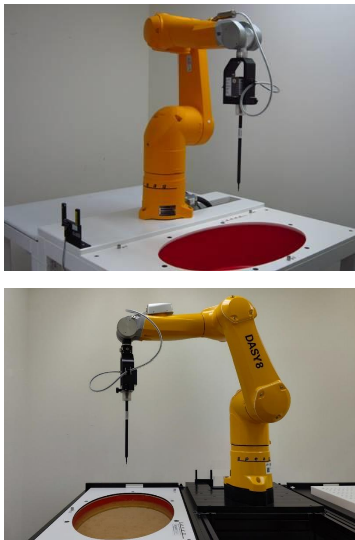
Fig.1 Photograph of the SAR measurement system
