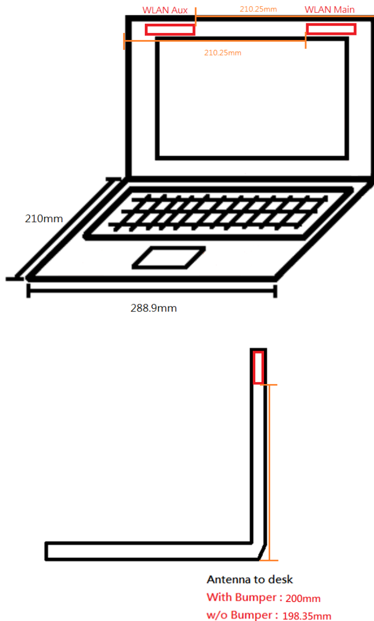
Photograph 17. Antenna position of EUT
