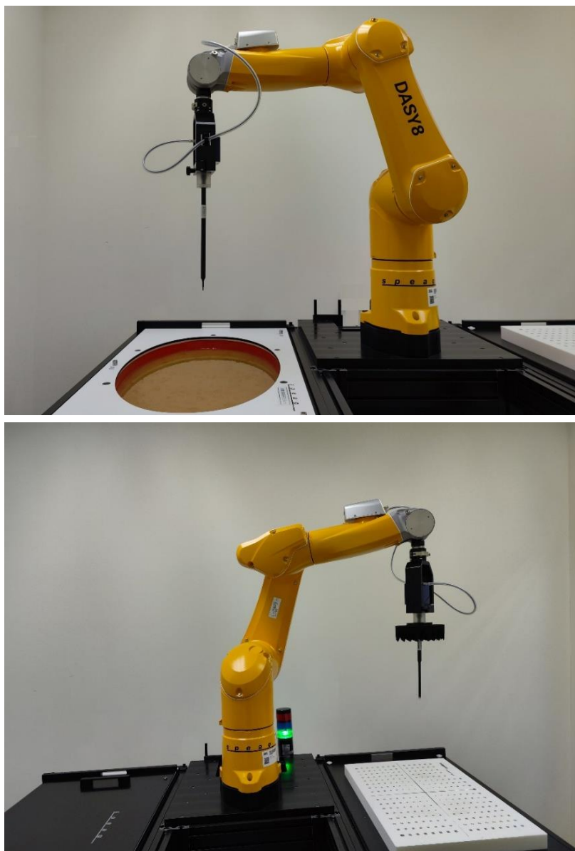
Fig.1 Photograph of the SAR measurement system
