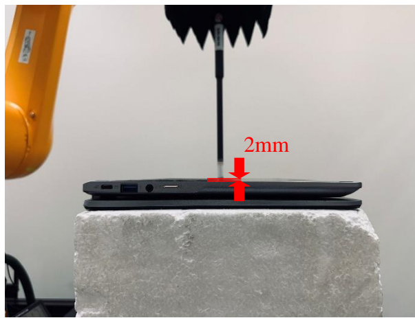
Photograph 12. PD, Back Surface, 2mm
