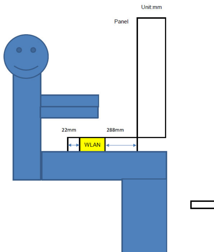
Photographs 6. Antenna position of EUT (Notebook mode)
