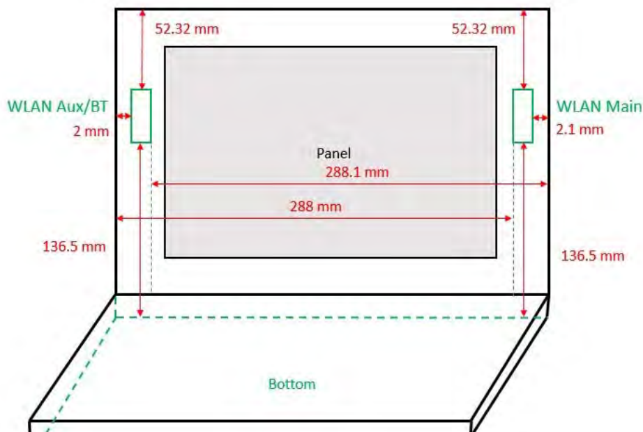
Fig.6 Antenna location of EUT (Notebook mode)
