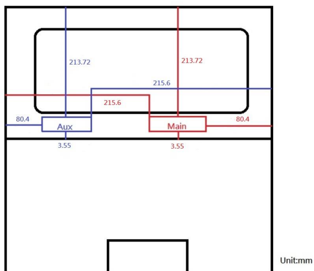
Fig.11 Antenna position of EUT
