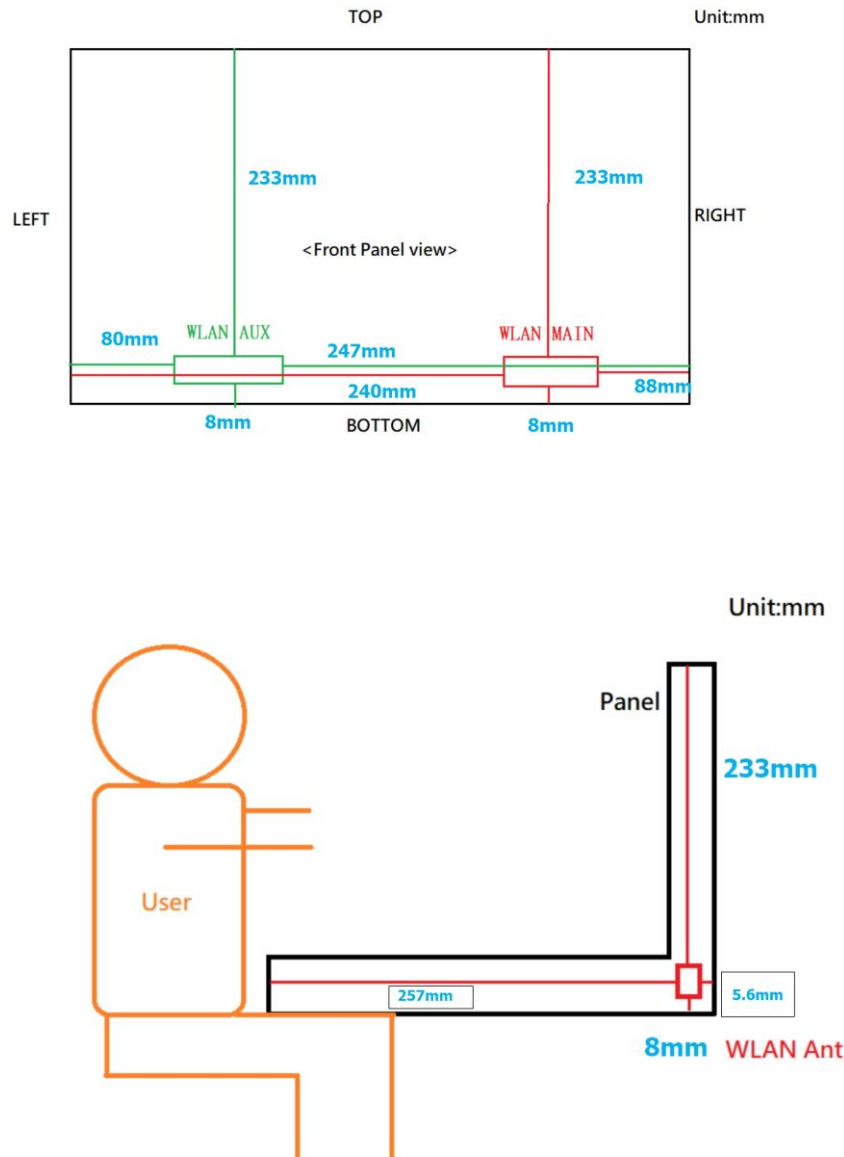
Fig.11 Antenna position of EUT
