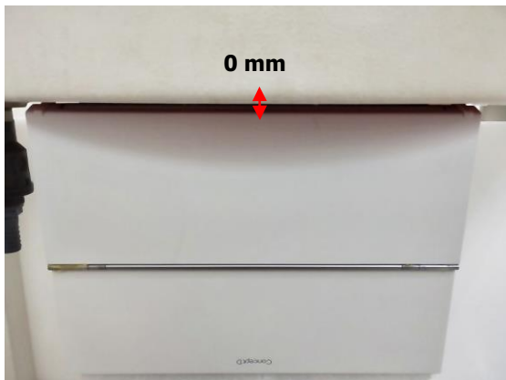
Fig.8 EUT Bottom side (NB mode) to flat phantom
