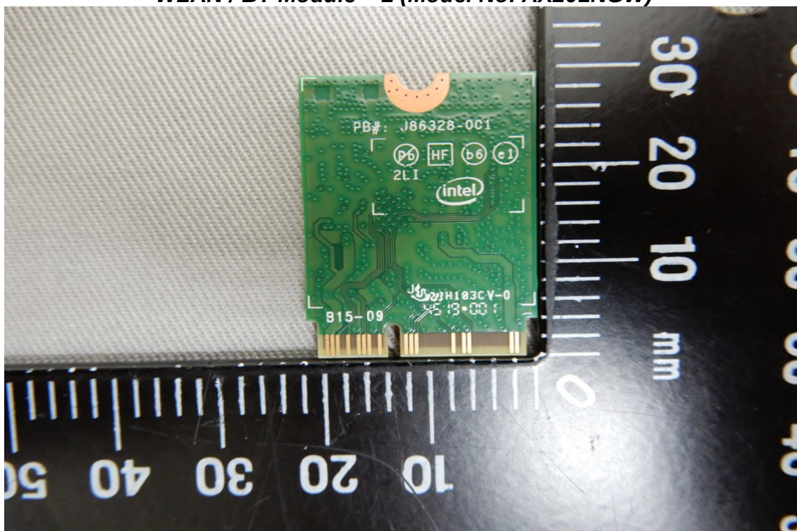
WLAN / BT Module – 2 (Model No: AX201NGW)
