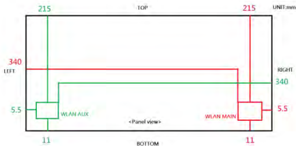
Fig.11 Antenna location of EUT (tablet mode)
