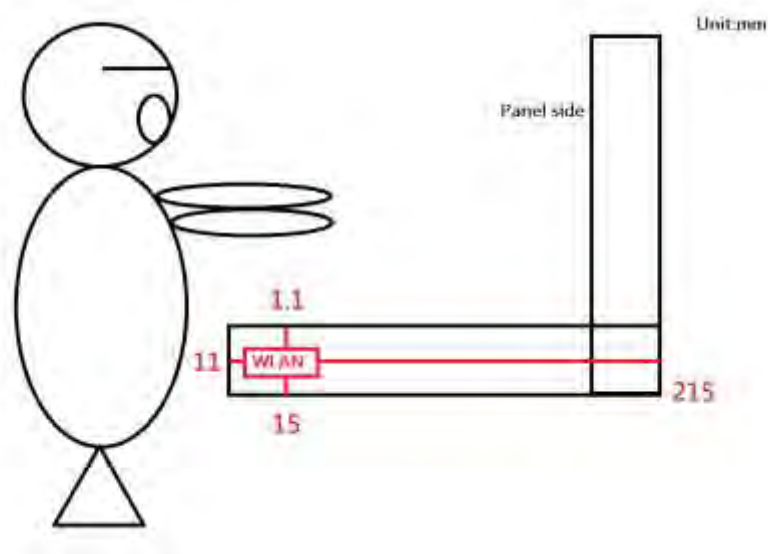
Fig.12 Antenna location of EUT (Notebook mode)
