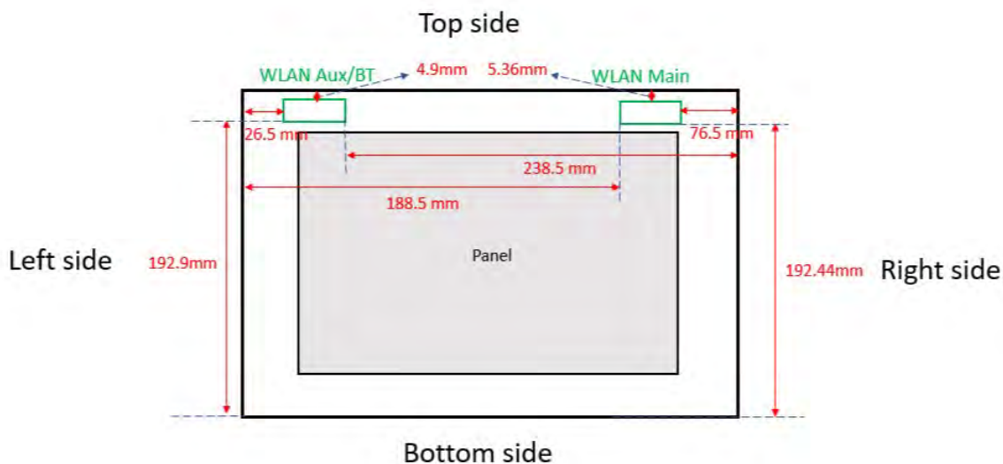
Fig.10 Antenna location of EUT (Tablet mode)
