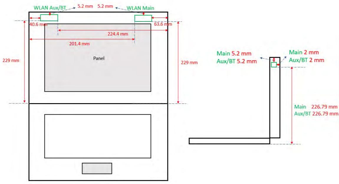
Fig.9 Antenna location of EUT (Tablet mode)
