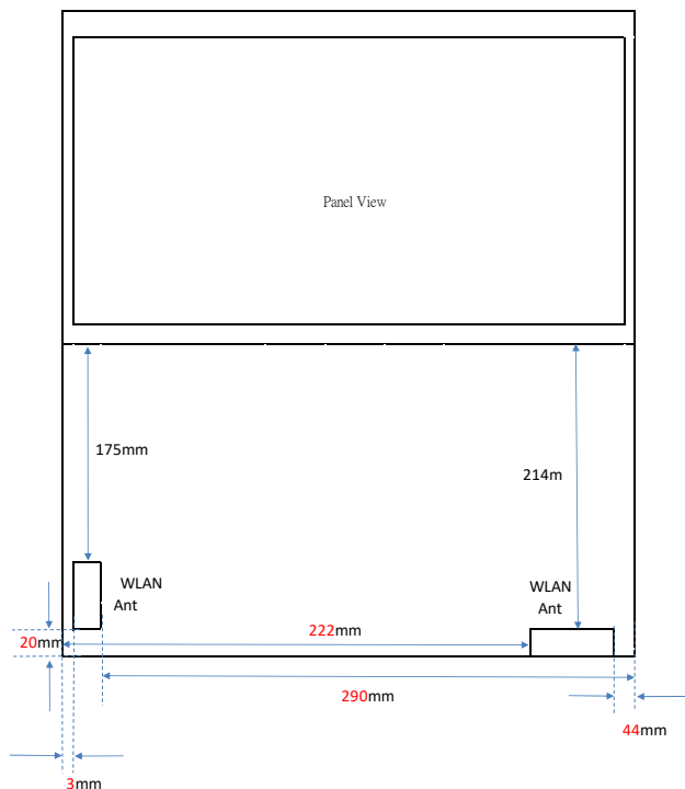
Photograph 5. Antenna position of EUT
