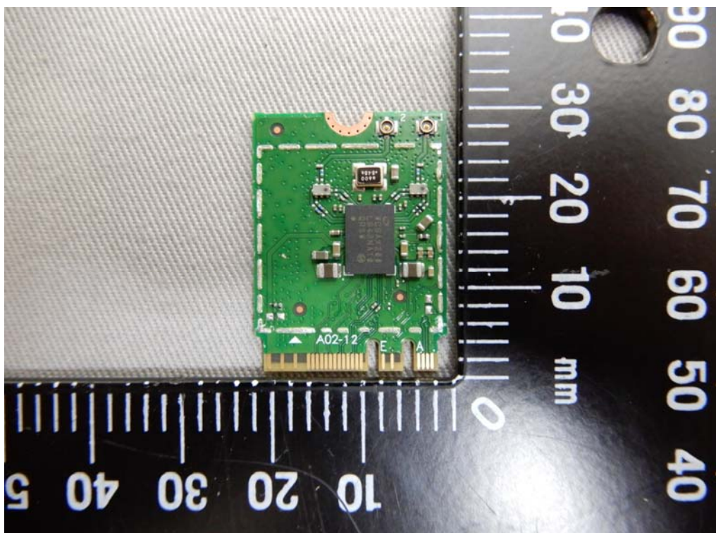
WLAN / BT Module - 3 (Model No.: AX200NGW)
