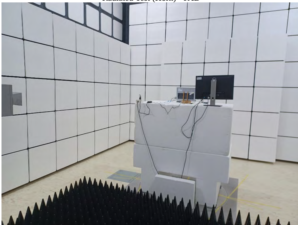
Radiated Test (Horn) - PAD
