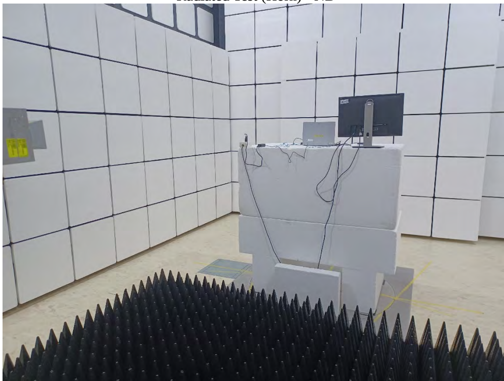
Radiated Test (Horn) - NB
