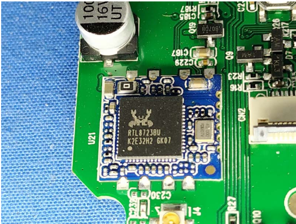
WIFI/BT module(Radio 2)
