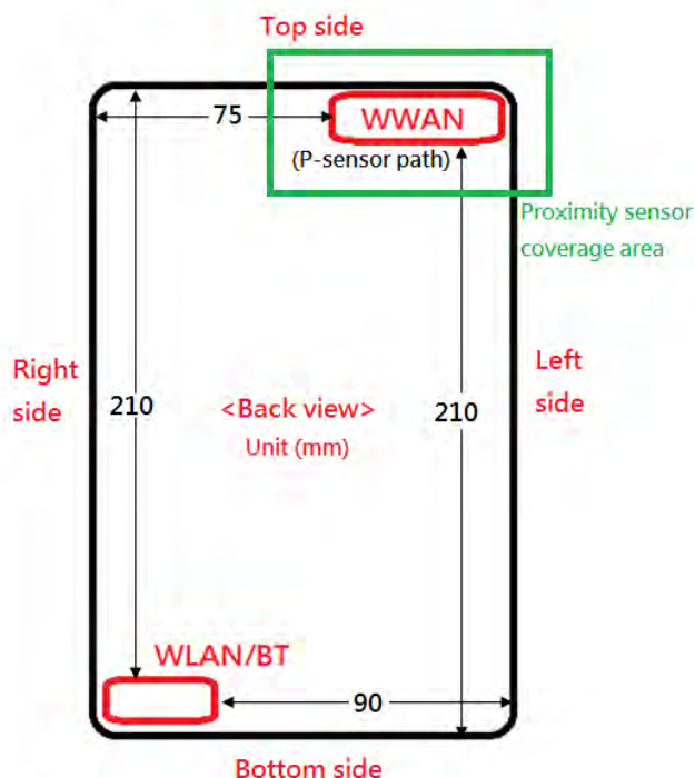
Fig.13 Antenna position of EUT (Front view)
